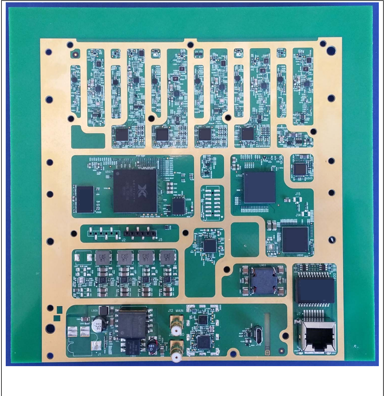
PCB Side 2 – no shield
