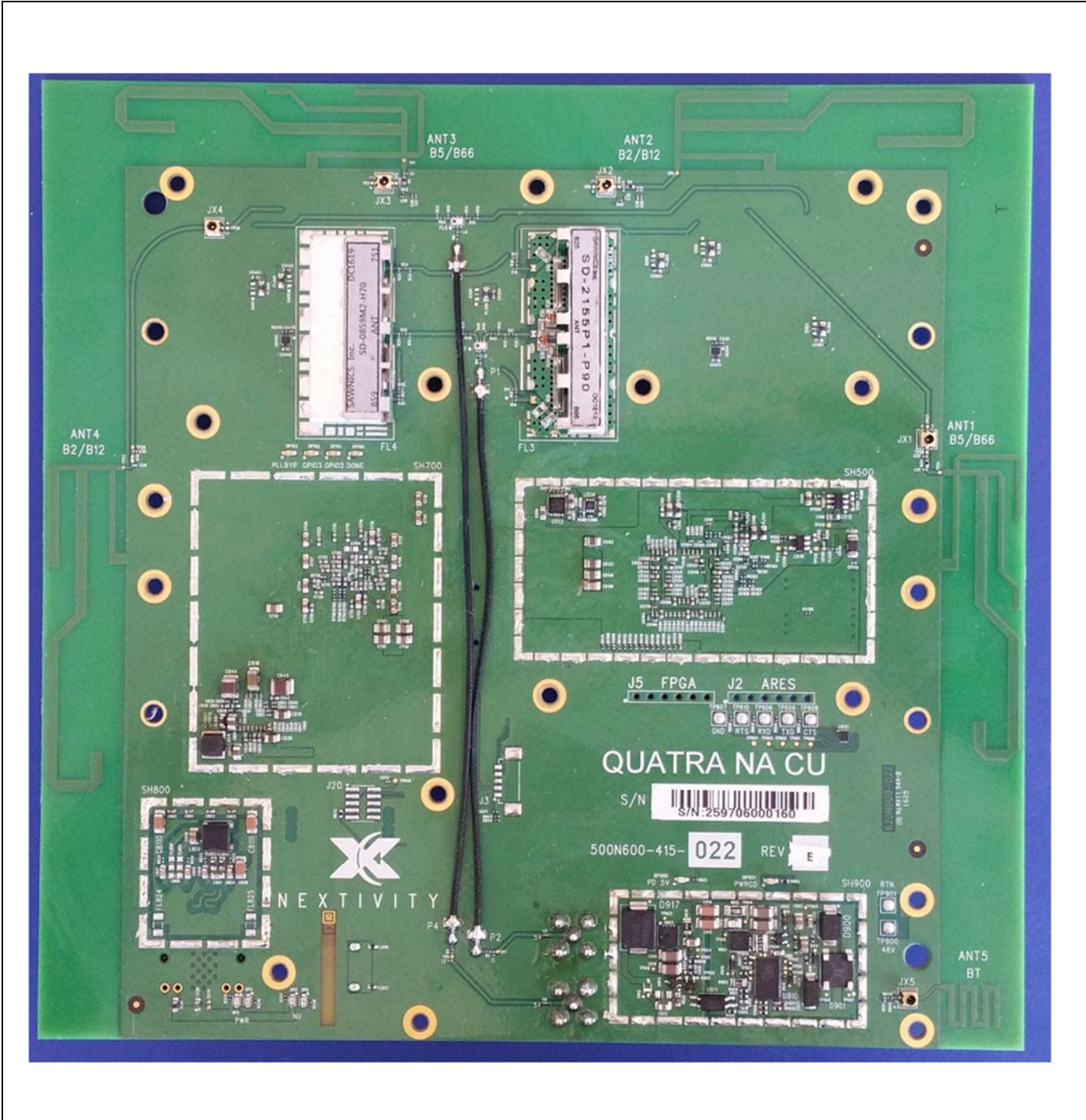
PCB Side 1 – no shield
