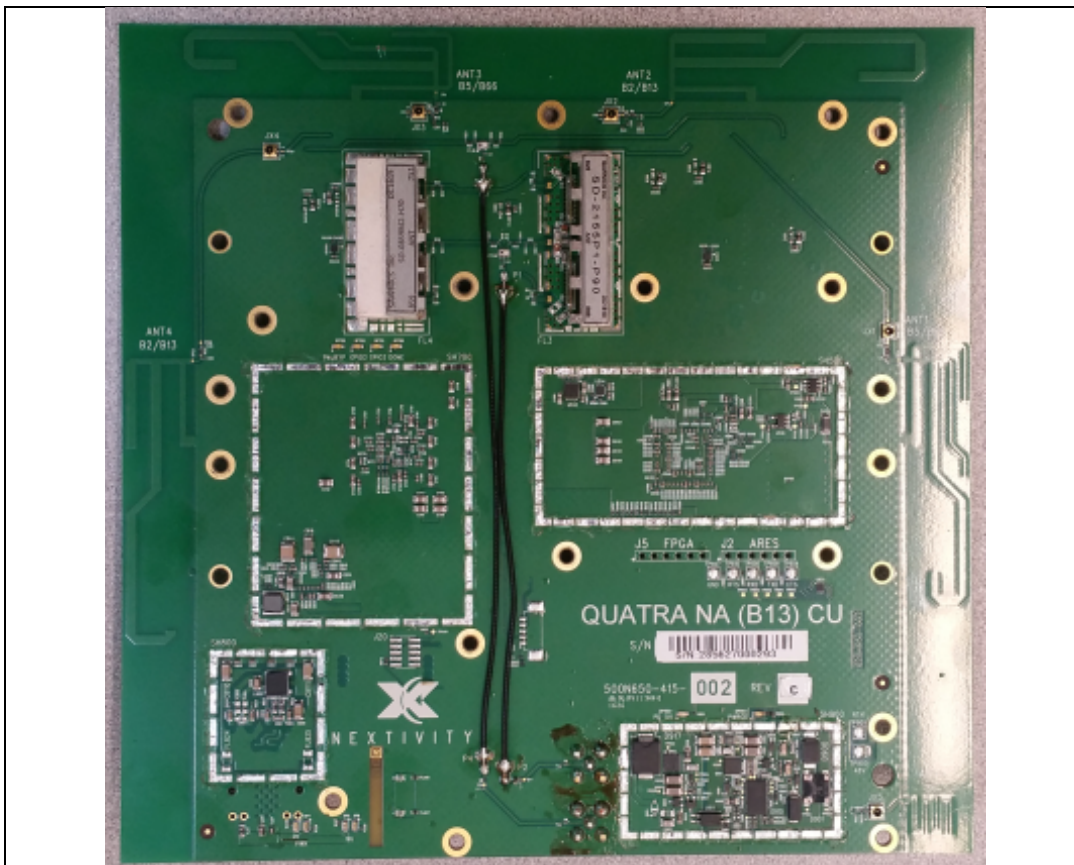
PCB Side 1 – no shield
