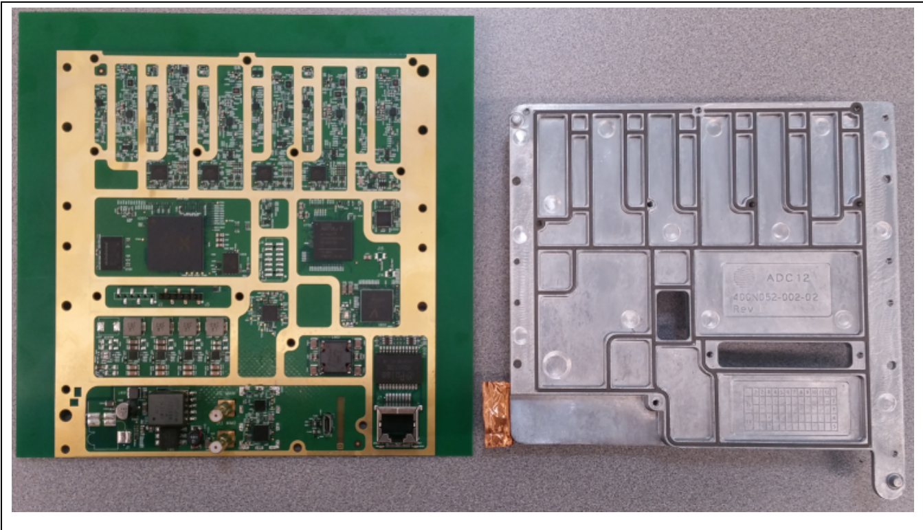
PCB Side 2
