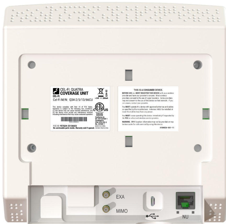
Label Location
