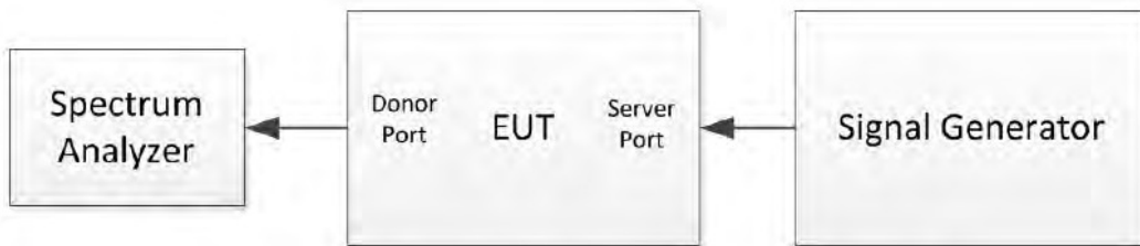
Figure 2: Uplink Test Configuration in Test Mode
