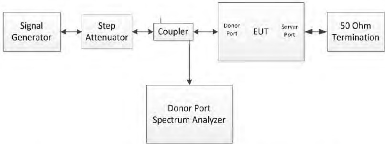
Figure 6: Uplink RSSI dependent noise limit test configuration
