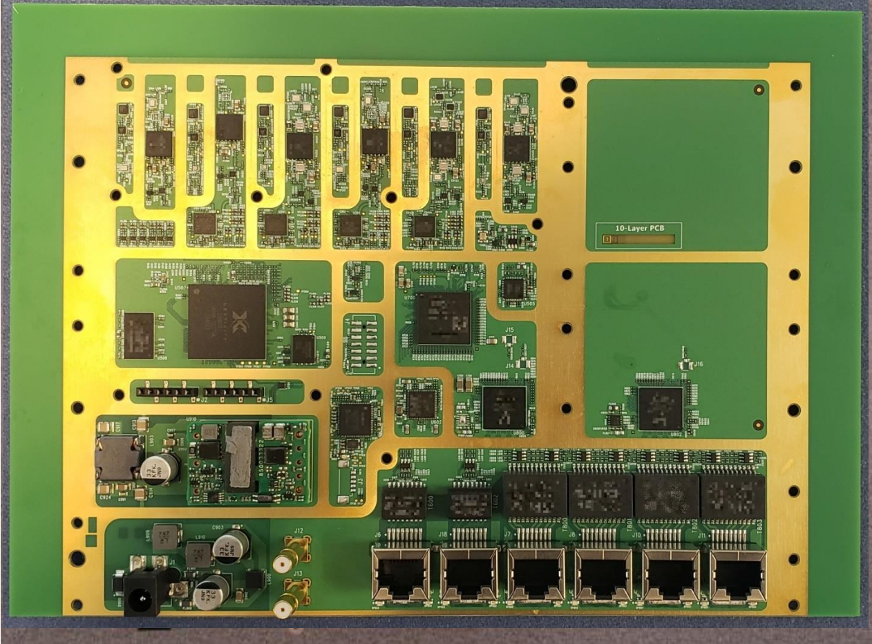
PCB Side 2
