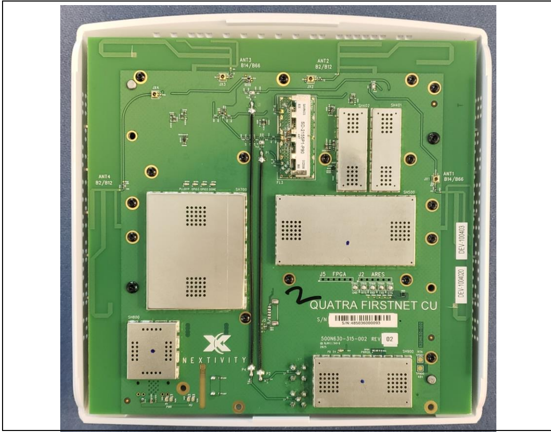
PCB Side 1
