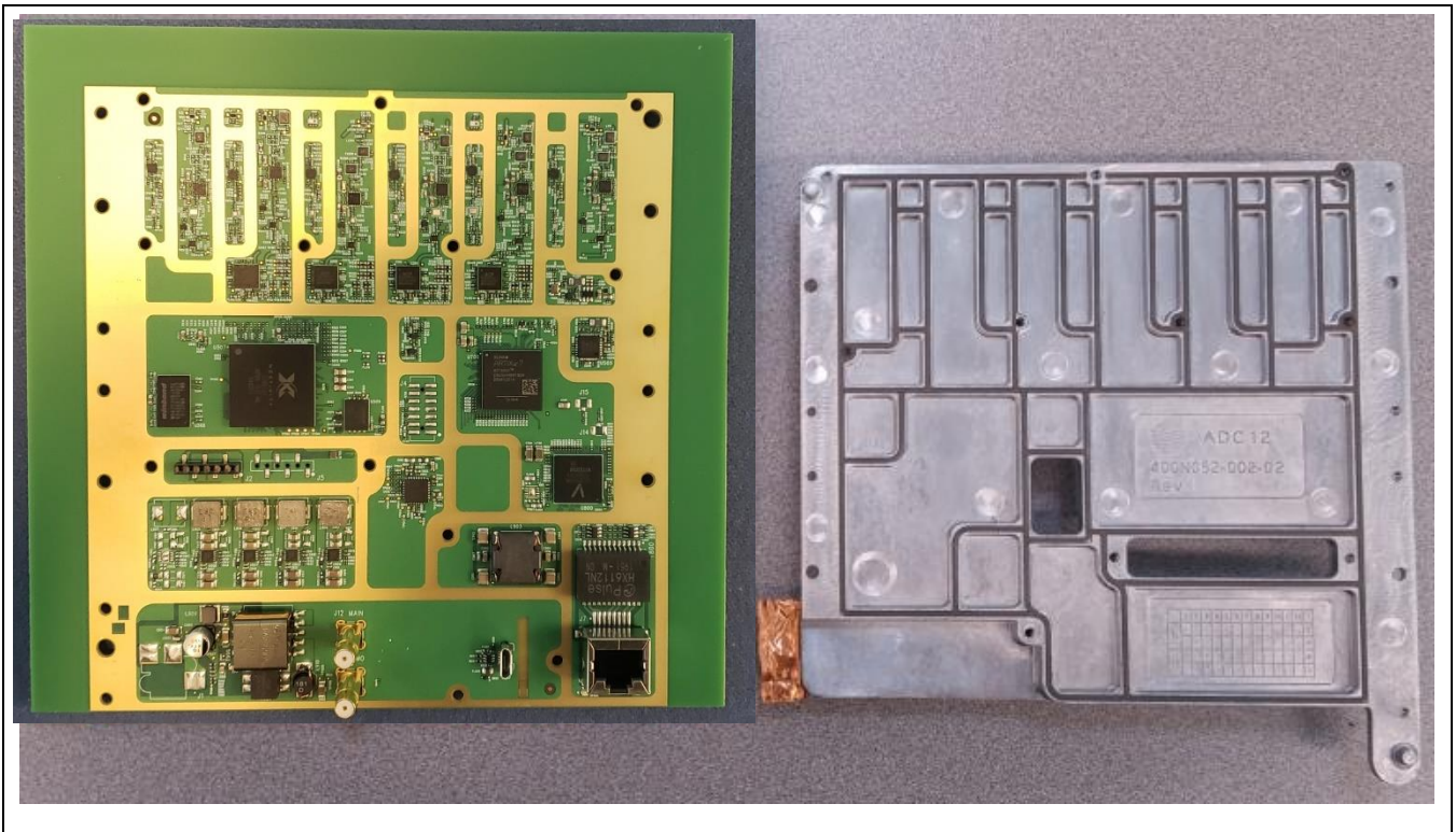
PCB Side 2
