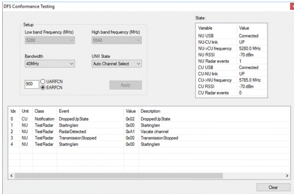
Configuration window showing original channels, radar detection at the end of CAC time and the alternative channel (5785 MHz) the CU moved to after NU detected the 5540 MHz Type 0 Radar
