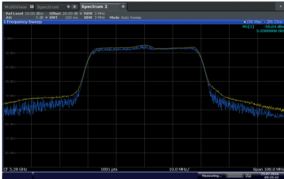
40 MHz BW 5280 MHz
