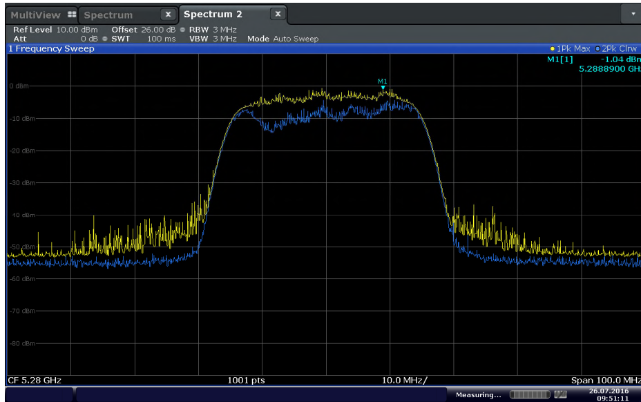
30 MHz BW 5280 MHz
