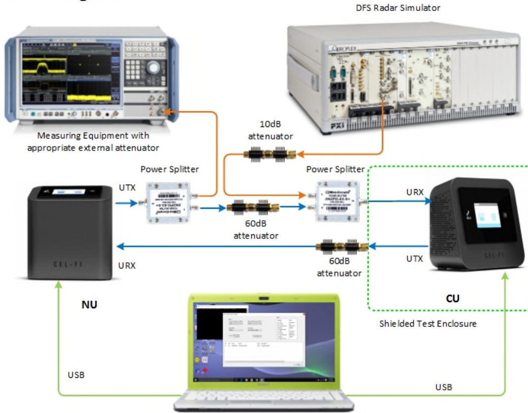
Support Laptop connected to both EUT via USB and running Nextivity DFS Conformance Test
