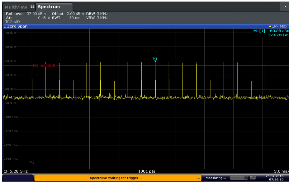
Radar Type 0 @ 5280 MHz
