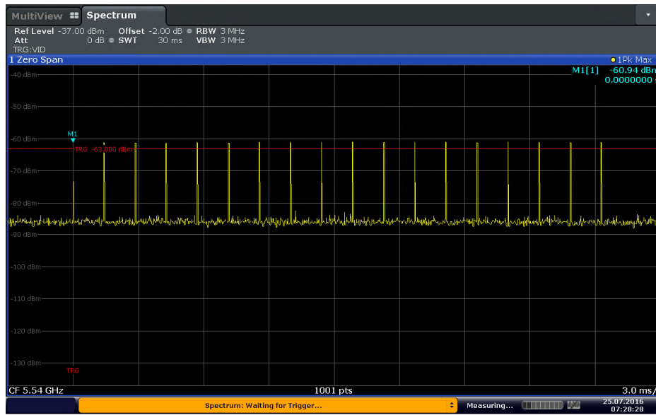
Radar Type 0 @ 5540 MHz
