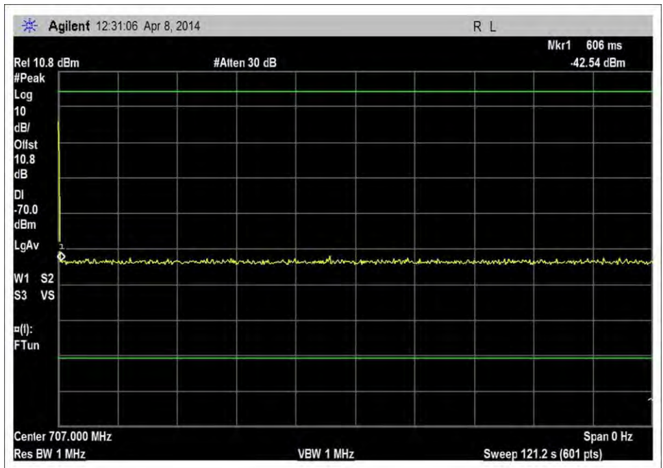
UL_698-716MHz_120s
