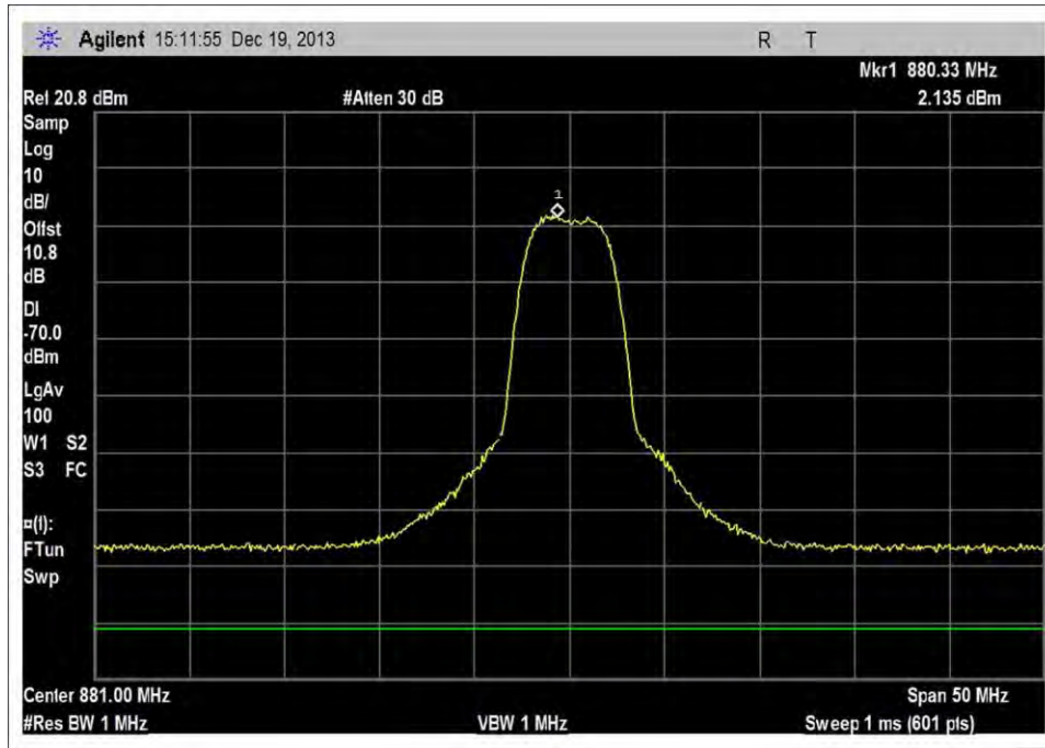
DL_869-894MHz_MNC410
