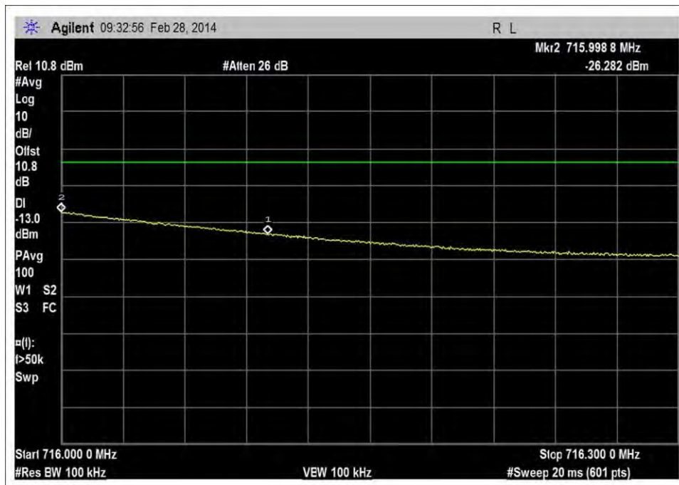
UL_698-716M-Hz_H_RFin _0dBm
