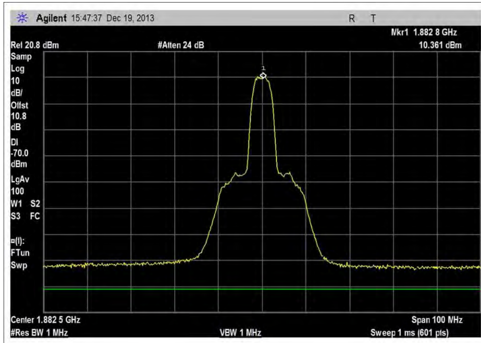
UL_1850-1915MHz_MNC410
