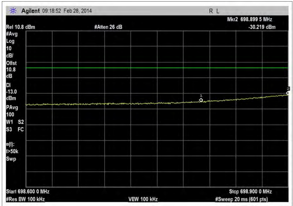
UL_698-716M-Hz_L_RFin -78dBm
