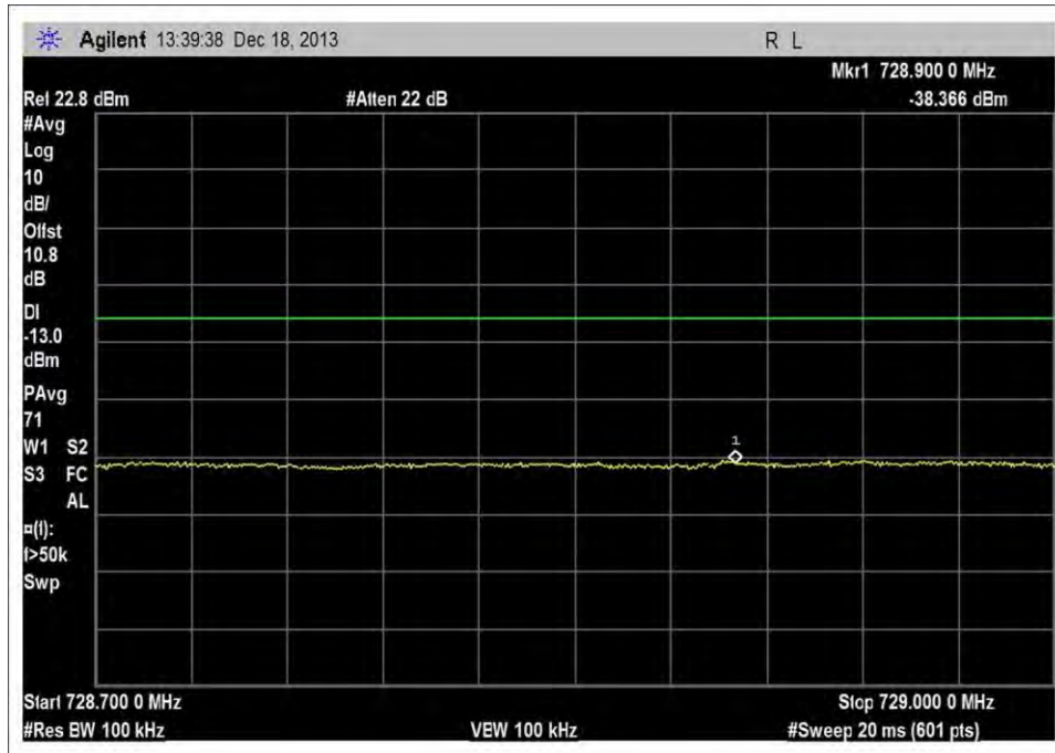
DL_716-746MHz_L_-20dBm
