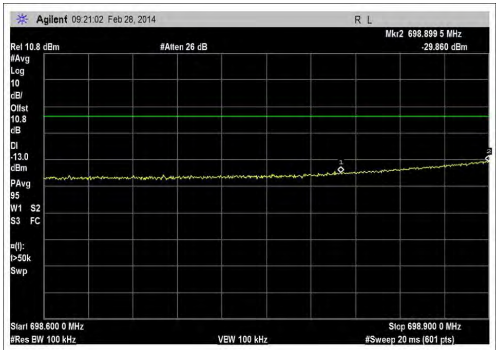
698-716M-Hz_L_RFin_0dBm
