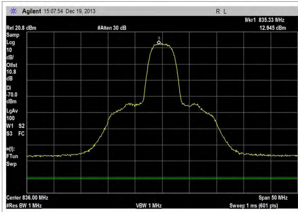
UL_824-849MHz_MNC410
