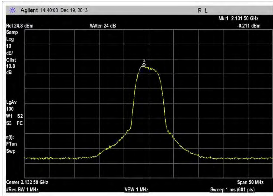
DL_2110-2155MHz_MNC410
