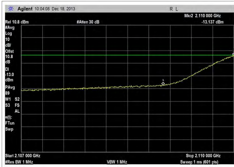
DL_2110-2155MHz_L_-20dBm
