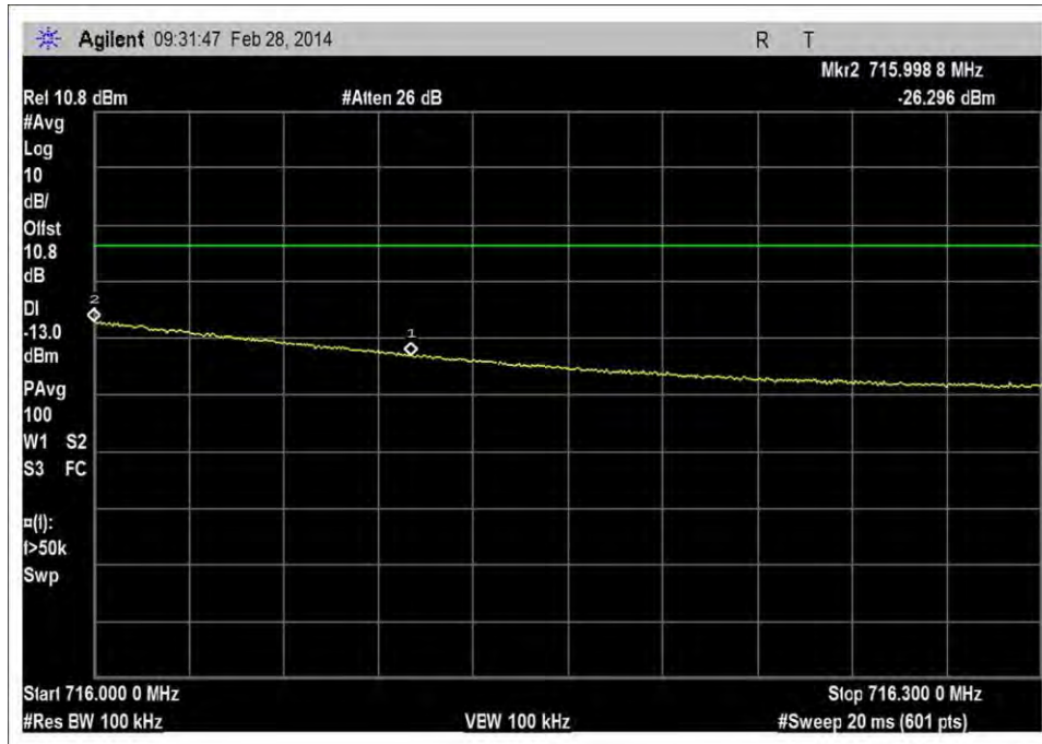
UL_698-716M-Hz_H_RFin -78dBm
