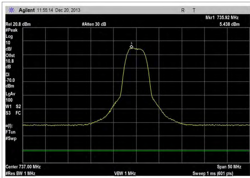
DL_716-746MHz_MNC410
