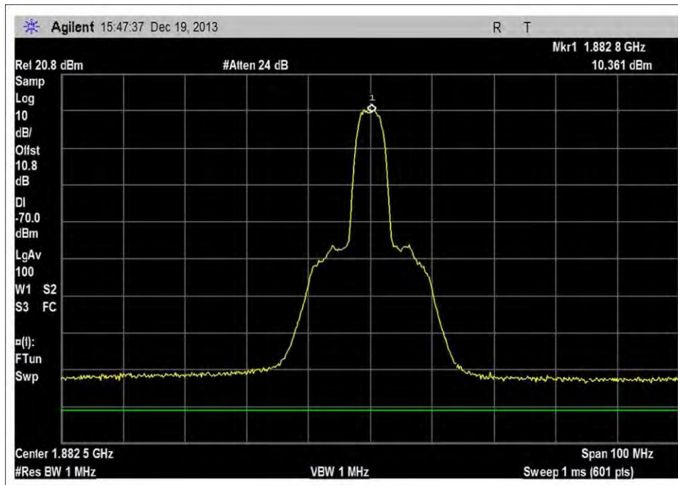
UL_1850-1915MHz_MNC410
