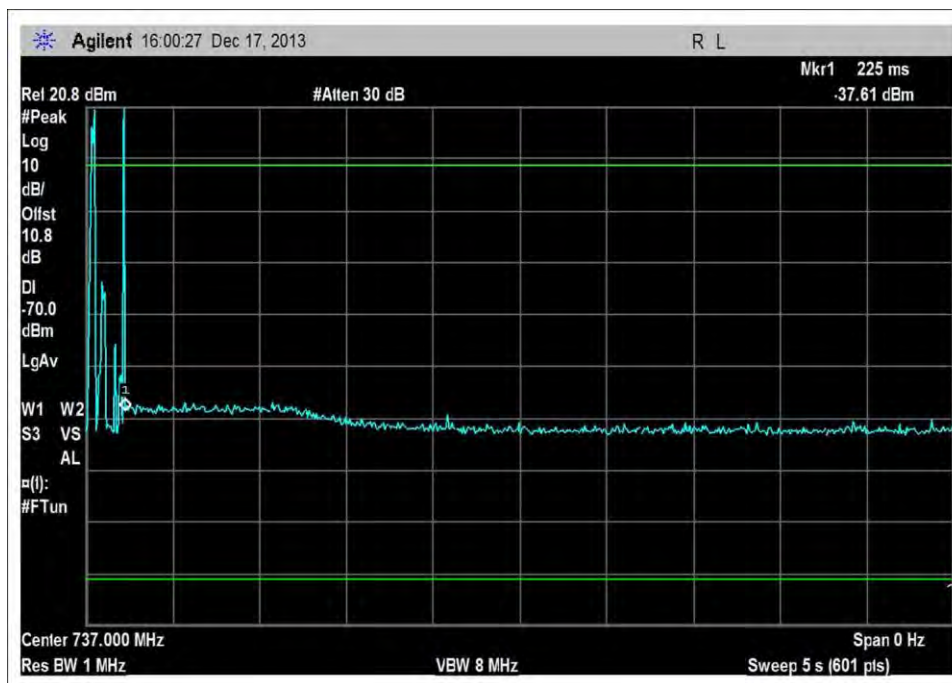
DL_716-746MHz_Single
