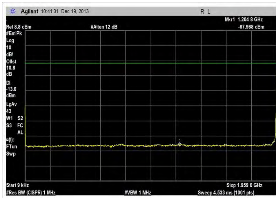
DL_1930-1995MHz_M_4.1AWGN_1
