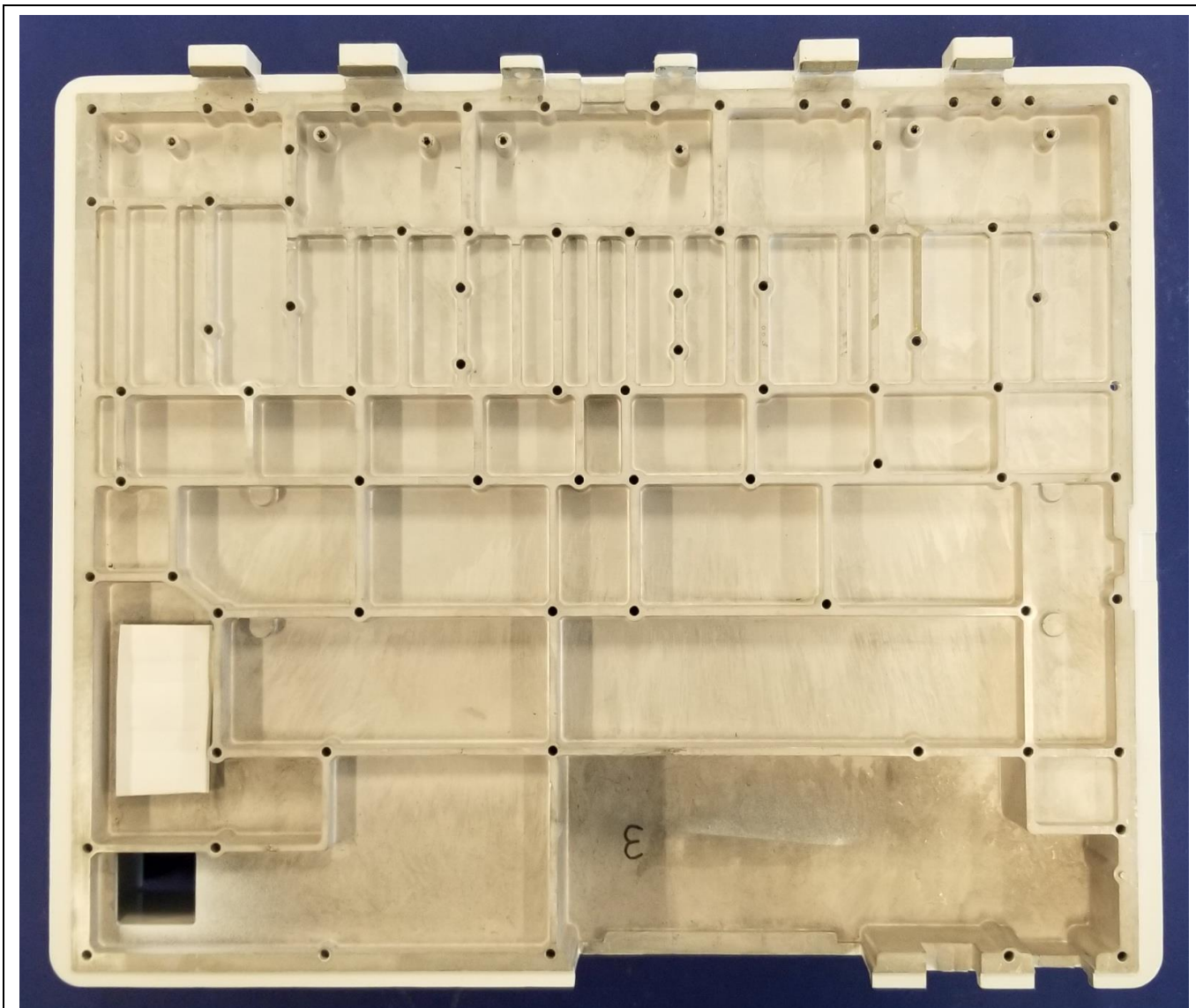
Housing_Bottom_Internal
