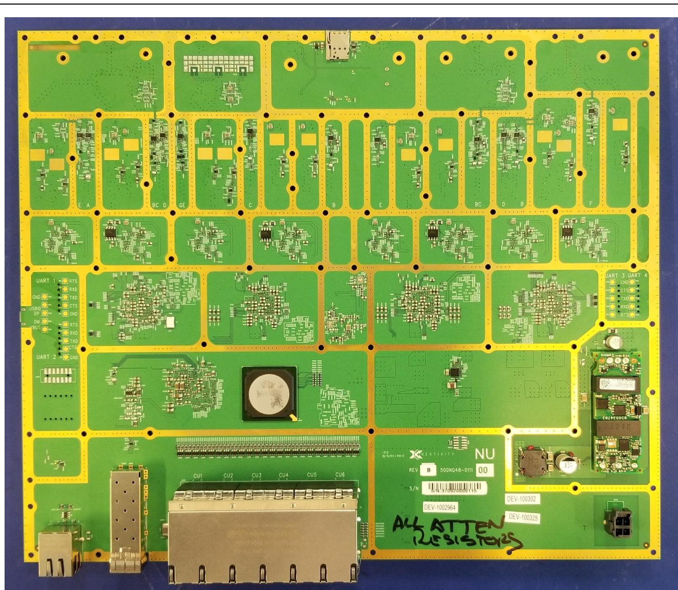
PCB side 2
