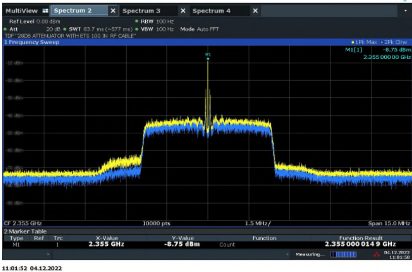
LTE B30 Downlink Middle Channel @ 40°C Nominal Voltage
