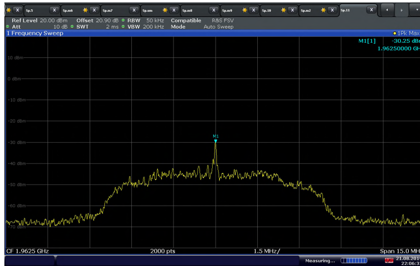
LTE B25 Downlink Middle Channel 120VAC @ 20°C
