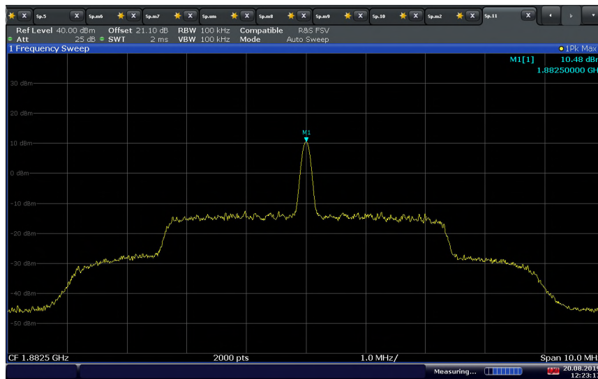
LTE B25 Uplink Middle Channel 120VAC @ 20°C
