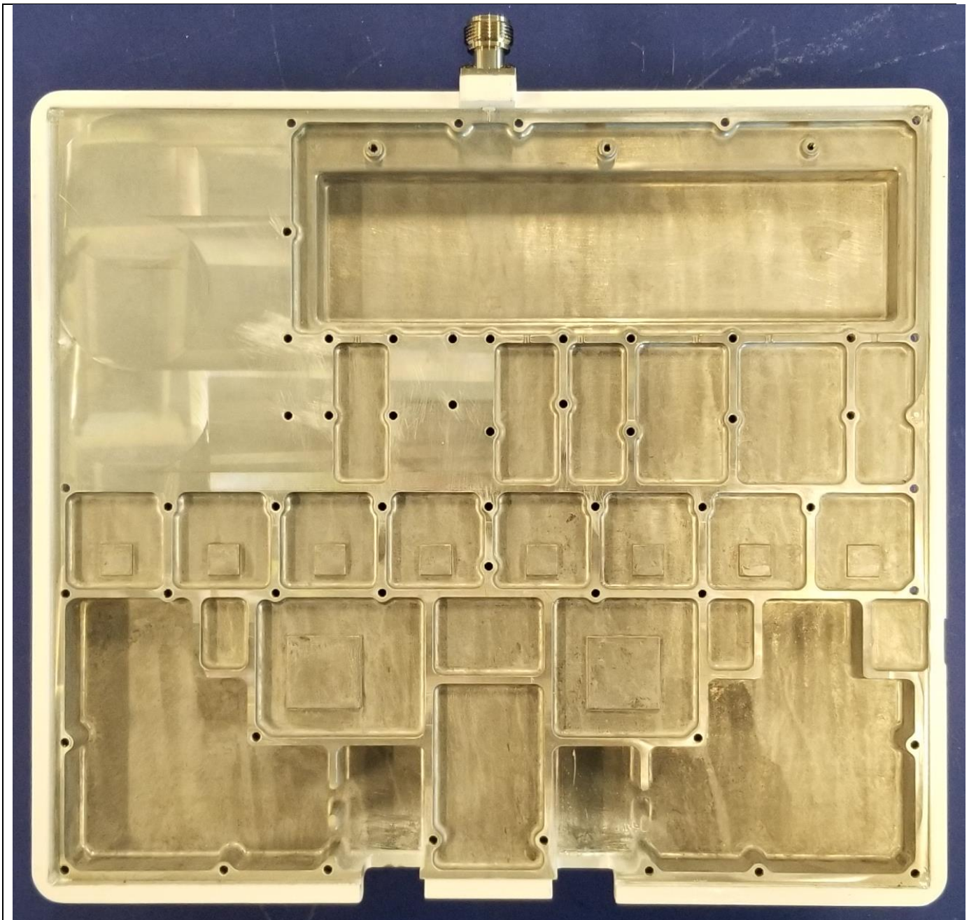
Housing_Bottom_Internal
