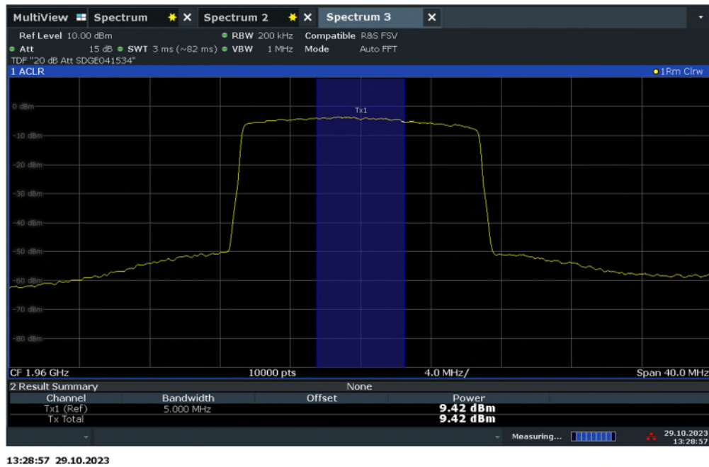
LTE Band 2 Downlink 10dBm/5MHz 15 MHz Bandwidth Middle Channel
