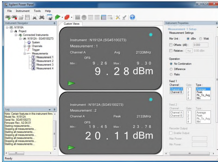
LTE Band 4 DL 5MHz Bandwidth Mid Channel
