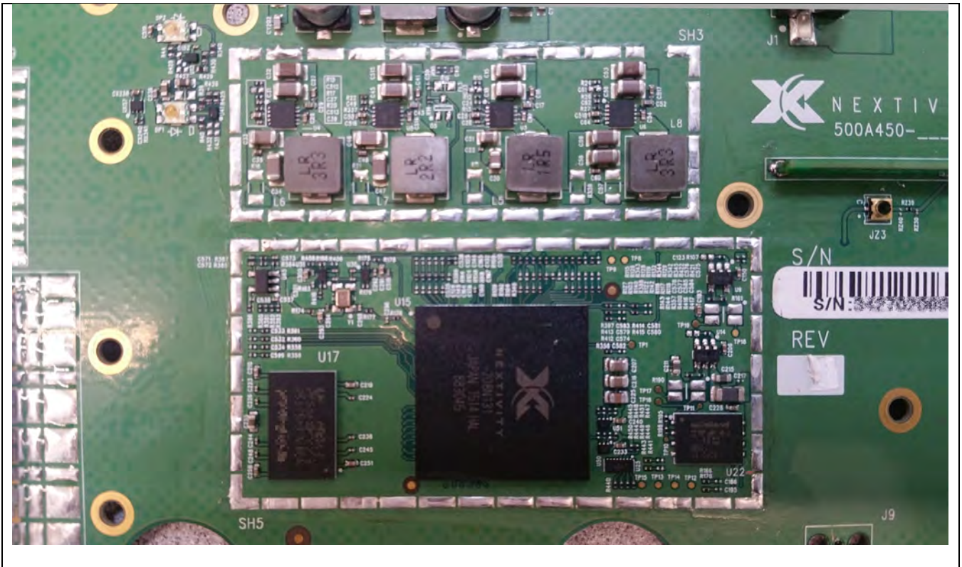
PCB - Top no shield Bottom
