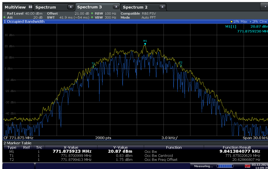
700MHz Narrowband Public Safety Downlink (C4FM 12.5 kHz BW) Mid Channel / 99% OBW at Output port with Input signal at AGC + 3 dB Level
