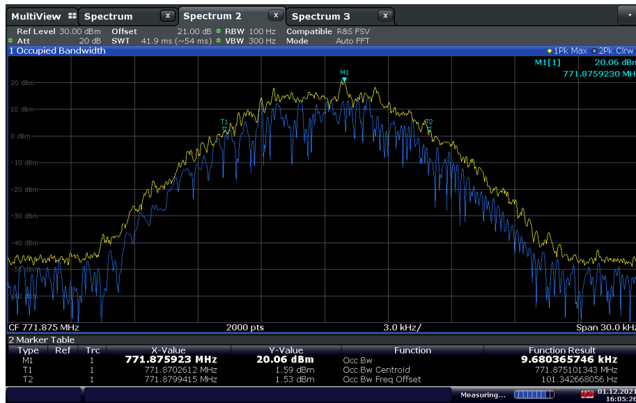
700MHz Narrowband Public Safety Downlink (C4FM 12.5 kHz BW) Mid Channel / 99% OBW at Output port with Input signal at AGC Threshold Level
