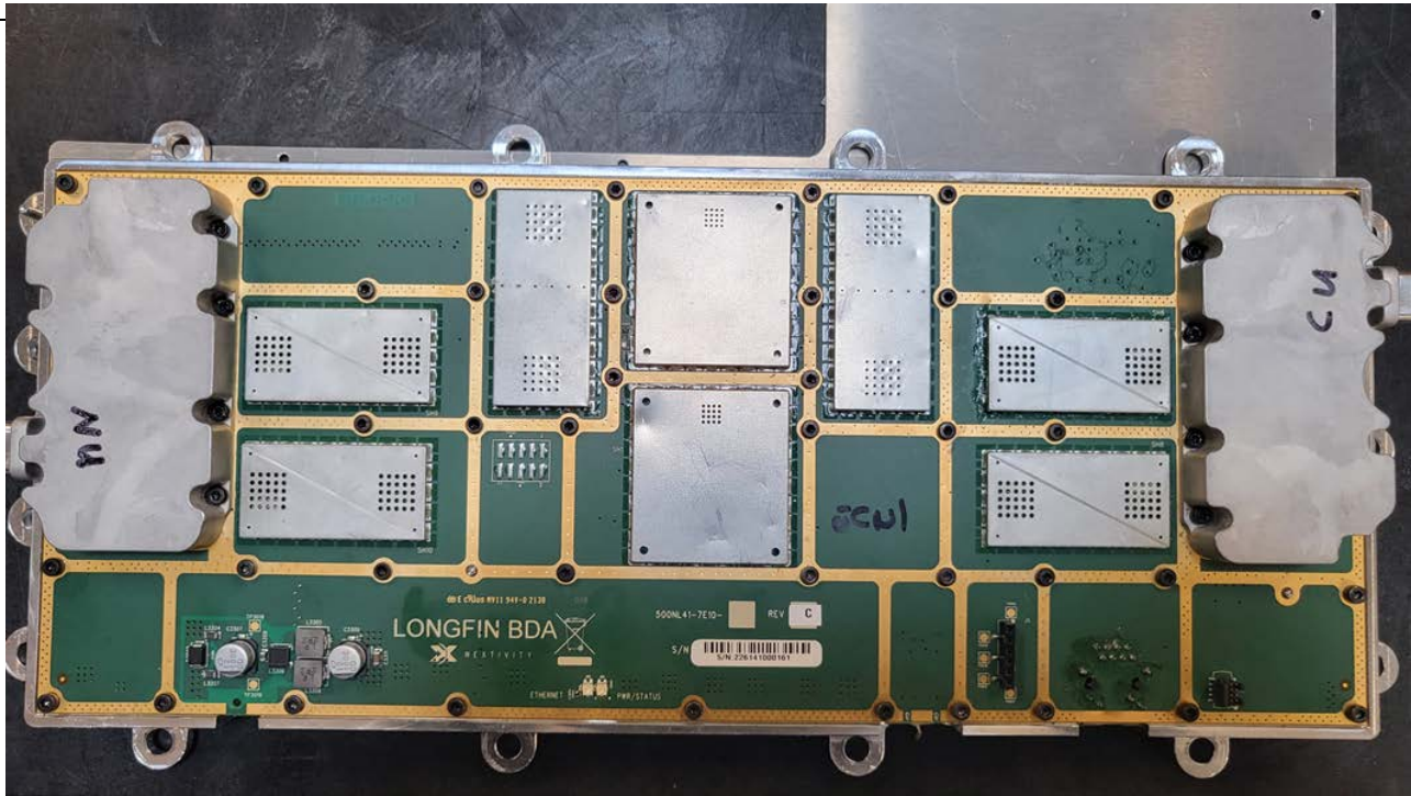
PCB_1 w/shields
