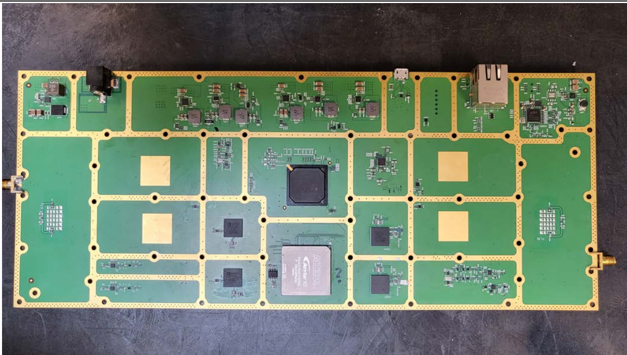
PCB_2
