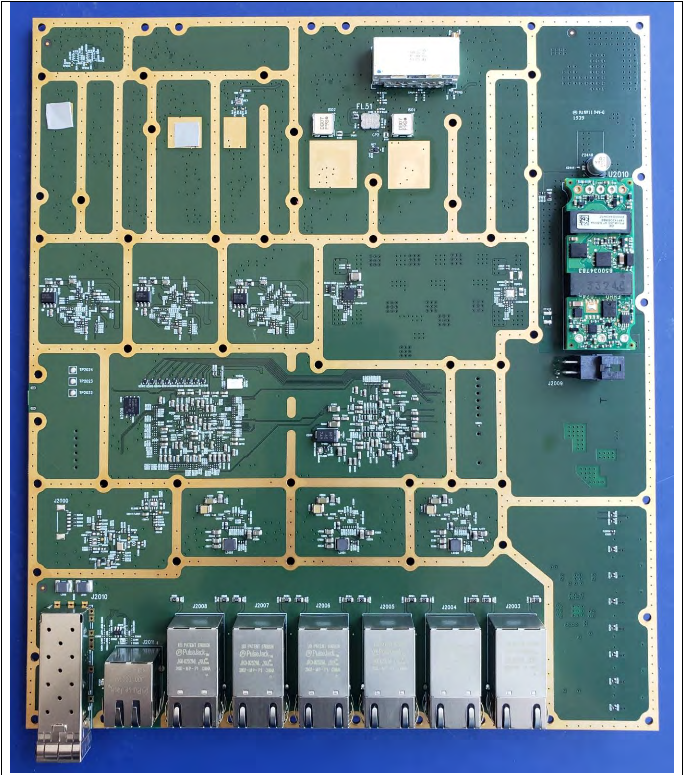
PCB side 2
