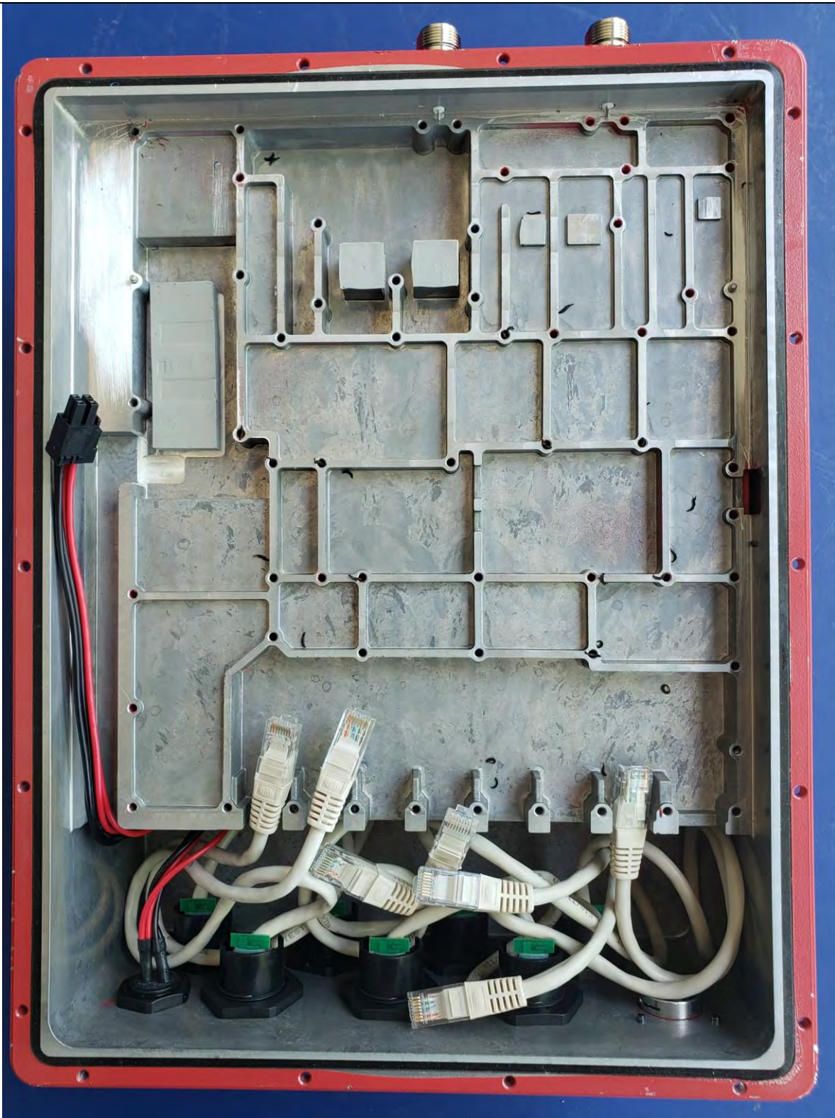
Housing, Bottom
