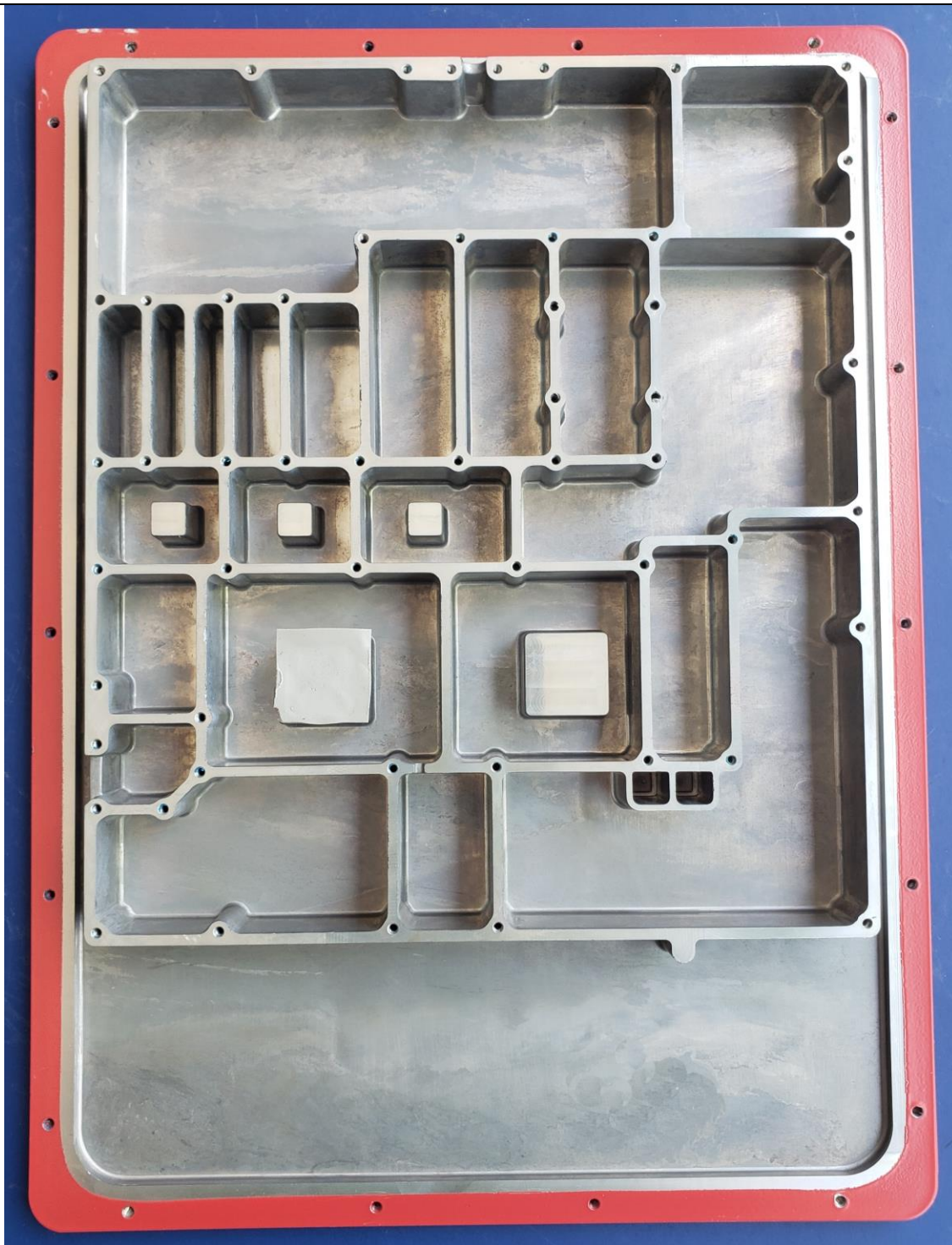
Housing_Top_Internal
