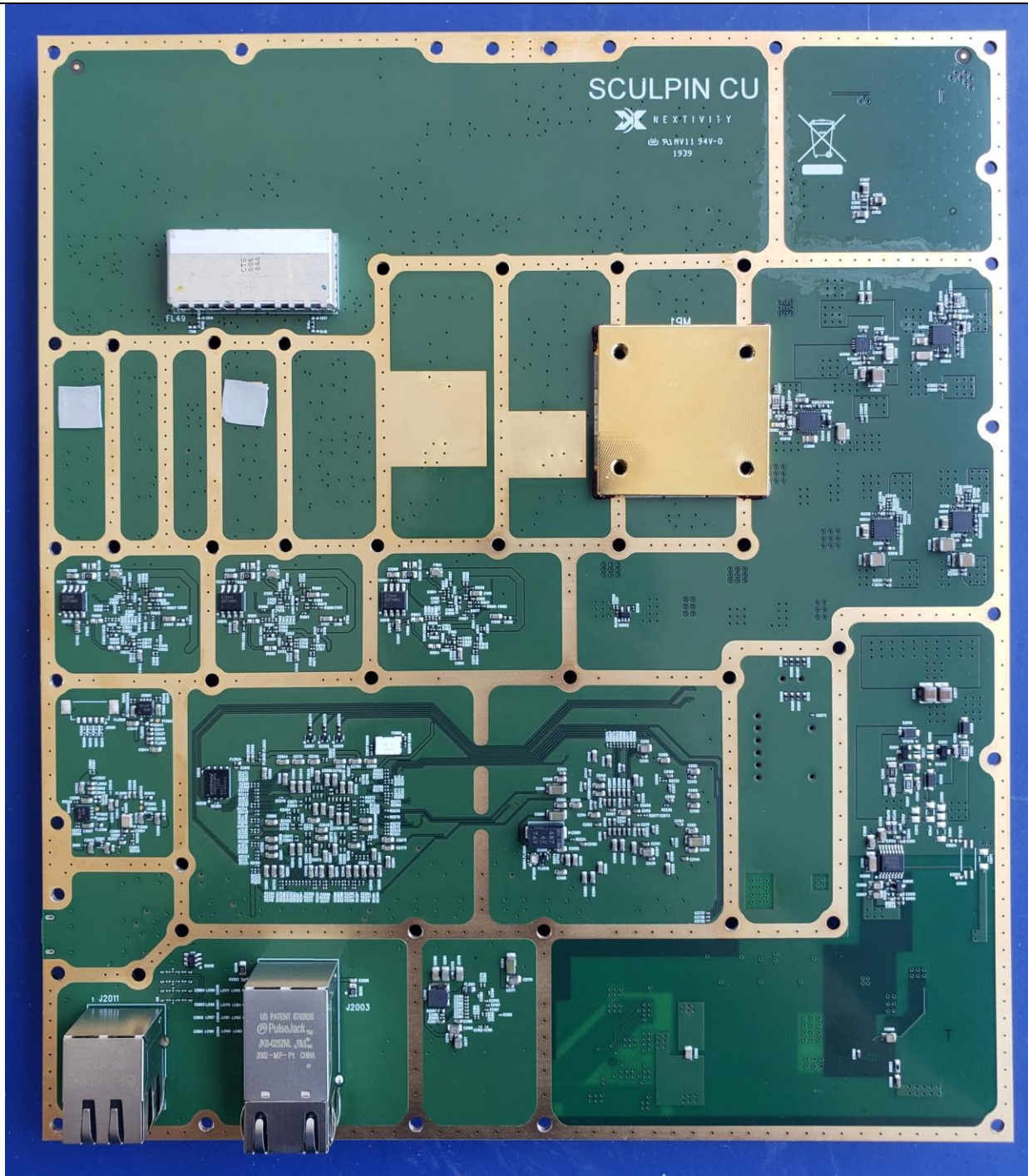
PCB side 2
