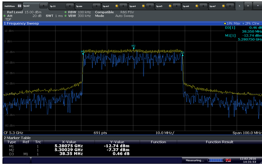
UNII 2A 40MHz Bandwidth Middle Channel 5300 MHz
