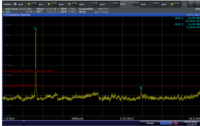
UNII 1 30MHz Bandwidth Middle Channel 5220 MHz Above 1GHz
