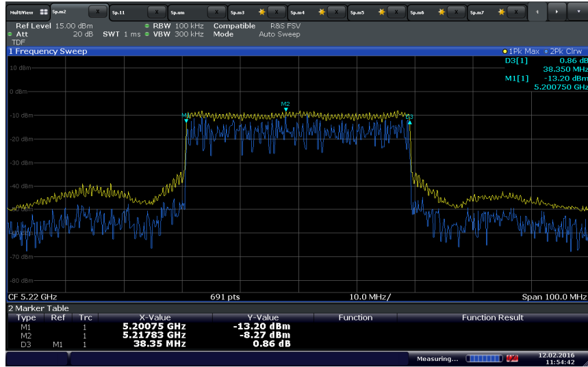
UNII 1 40MHz Bandwidth Mid Channel 5220 MHz
