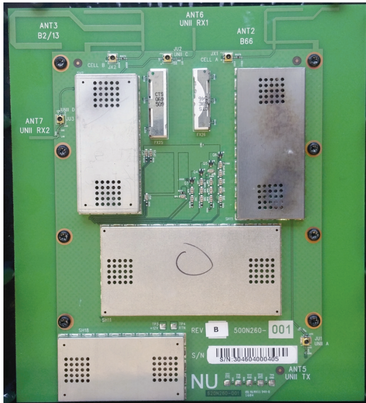
PCB Side_1 – NU
