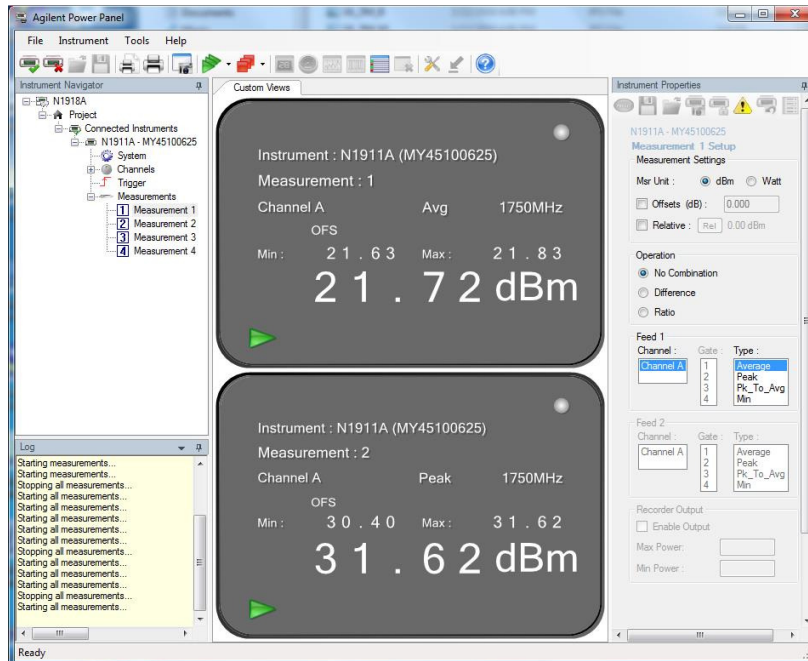
LTE Band 66 UL 5MHz Bandwidth Mid Channel
