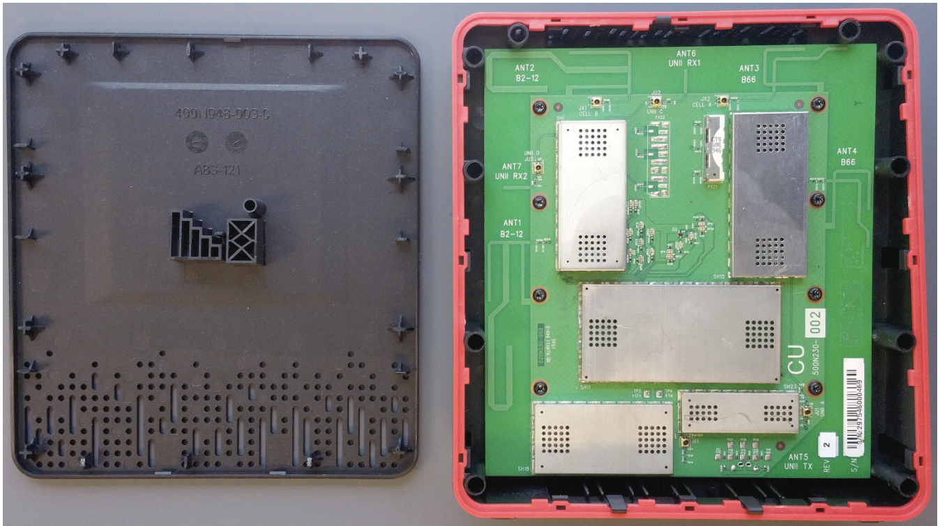
Housing_1 – CU
