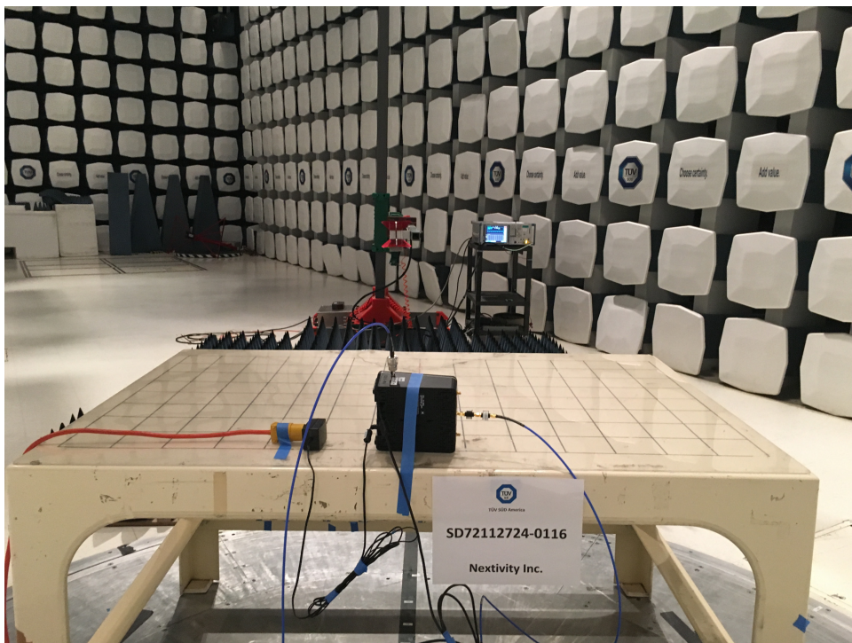
Radiated Emissions
