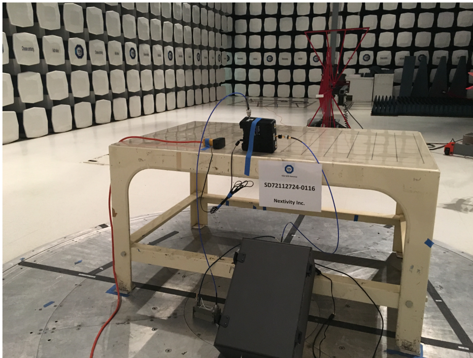
Radiated Emissions
