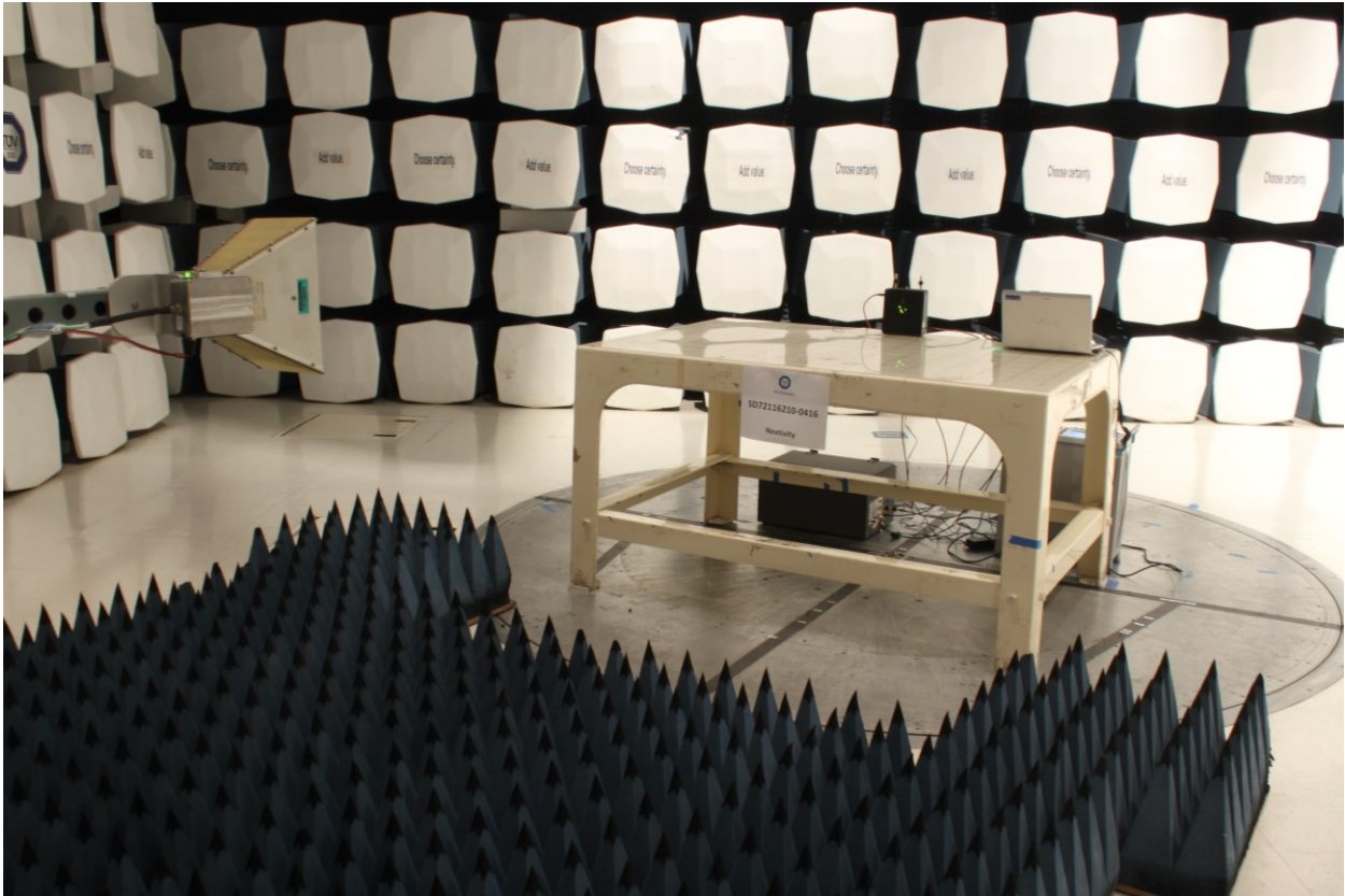
Radiated Emissions
