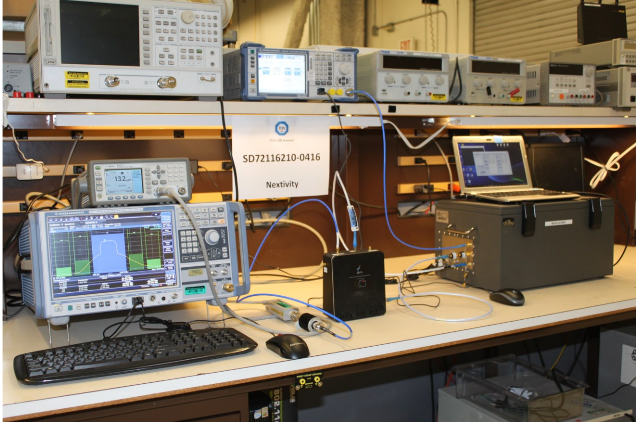
Conducted Testing
