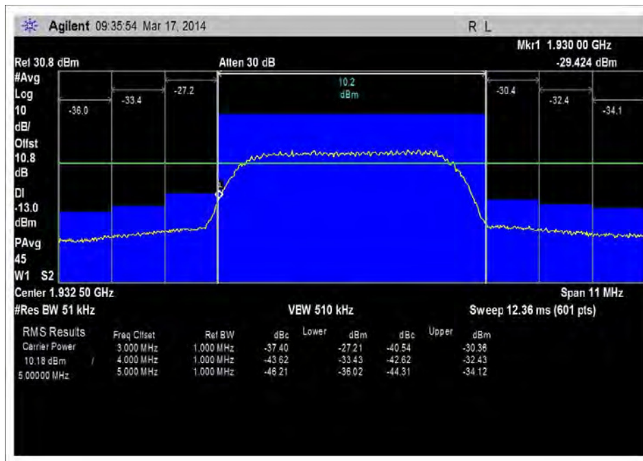
DL 1930-1995MHz, cursor set at 1930MHz. Channel power 1 MHz outside the band is -27.2dBm
