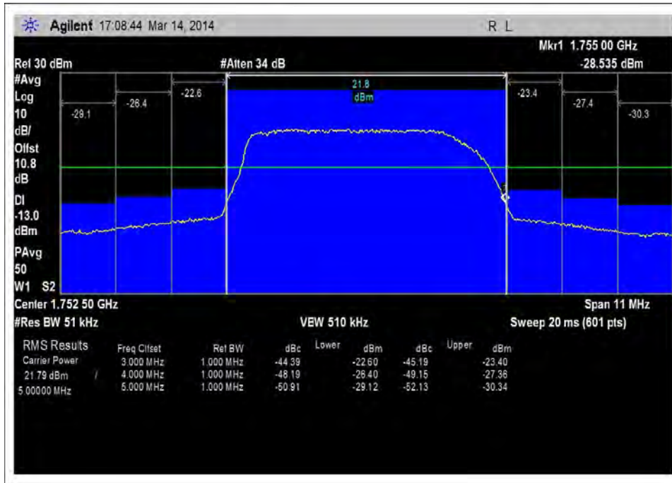
UL 1710-1755, cursor set at 1755MHz. Channel power 1 MHz outside the band is -23.4dBm
