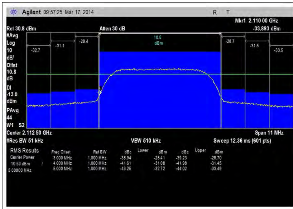
DL 2100-2155MHz, cursor set at 2110MHz. Channel power 1 MHz outside the band is -28.4dBm
