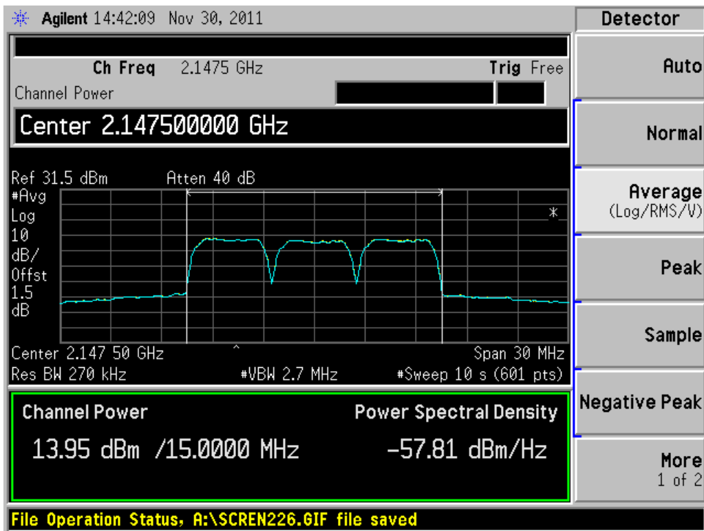
Figure 2 - Average Power
