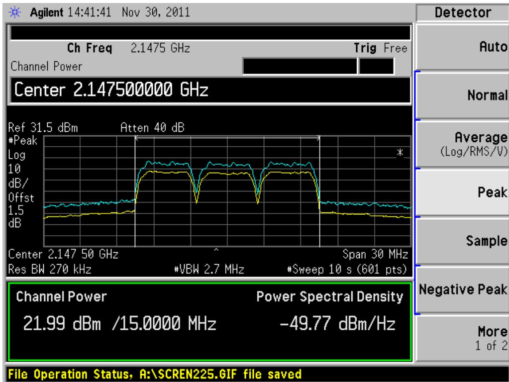
Figure 1 - Peak power
