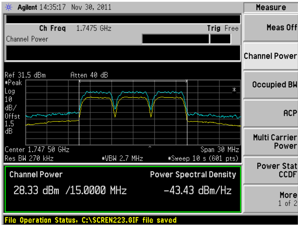
Figure 1 - Peak power
