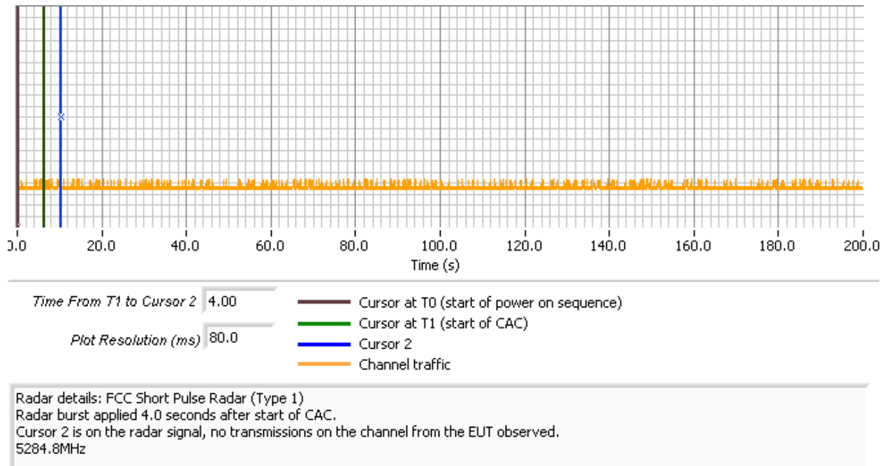
Figure 20 Radar Applied At Start of CAC, WU Low Band
