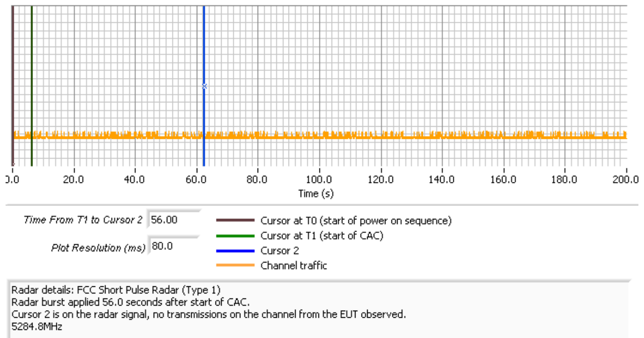
Figure 21 Radar Applied At End of CAC, WU Low Band
