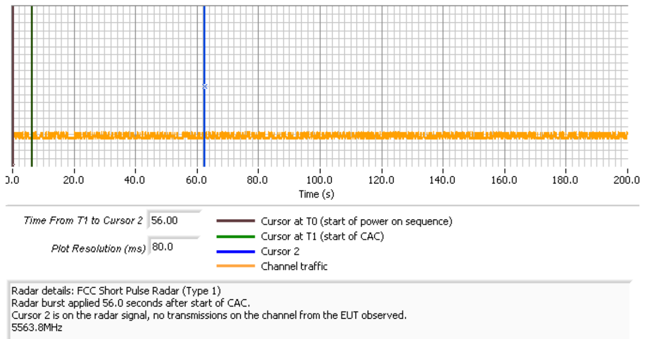
Figure 23 Radar Applied At End of CAC, WU High Band
