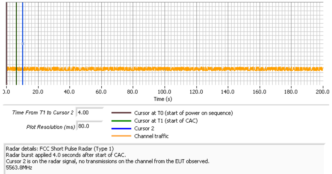
Figure 22 Radar Applied At Start of CAC, WU High Band
