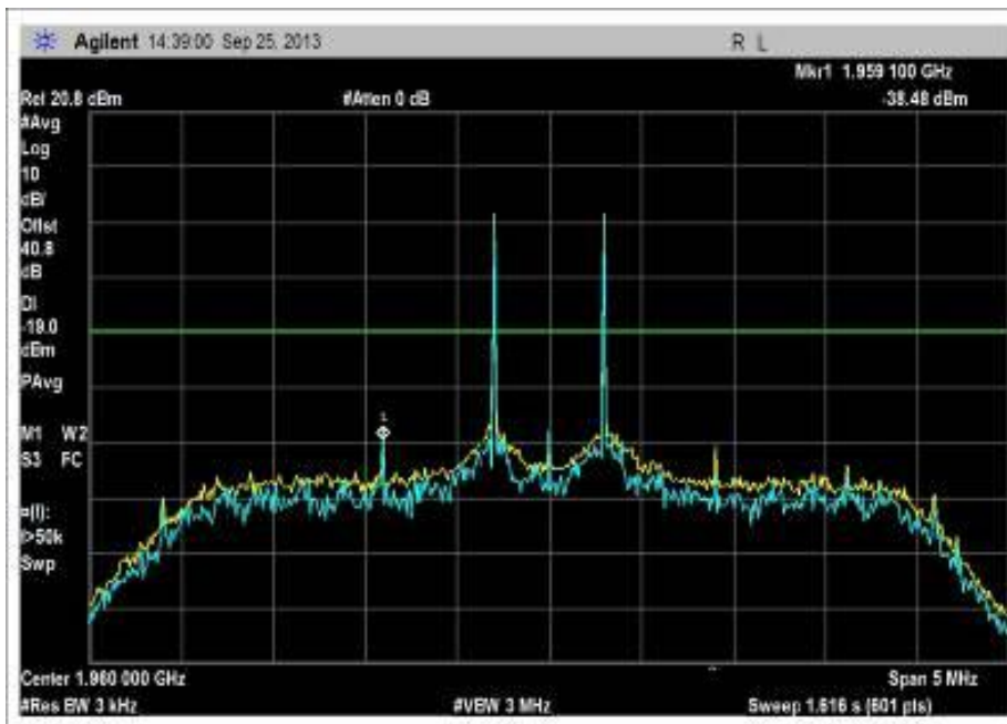
7.4 intermod_1930-1990MHz
