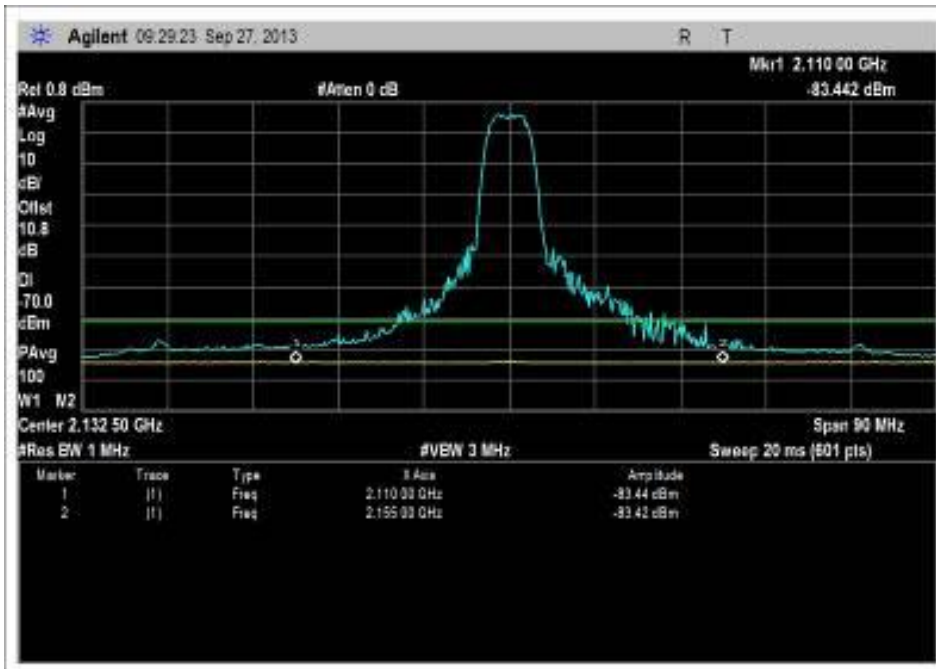
DL: 2110-2155MHz Blue trace is Booster on, signal in the center of the band is the DL signal. Yellow trace is DL noise power in the absent of DL signal.
