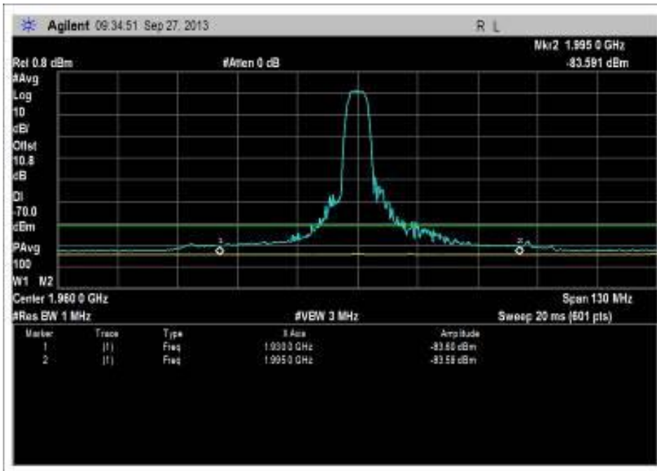
DL: 1930-1990MHz Blue trace is Booster on, signal in the center of the band is the DL Signal. Yellow trace is DL noise power in the absent of DL signal.
