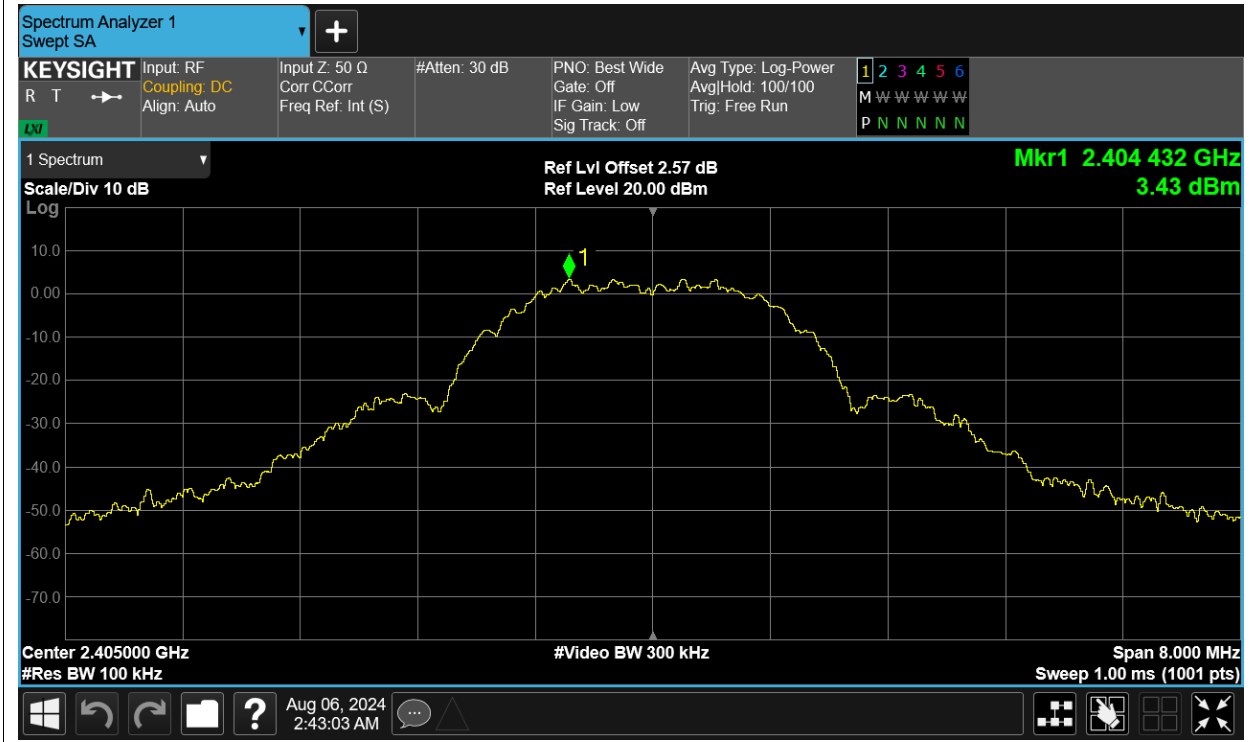
Band Edge NVNT ZigBee 2405MHz Ant3 Emission
