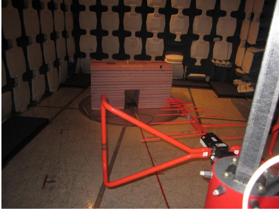
Radiated Emission - Front 30-1000MHz
