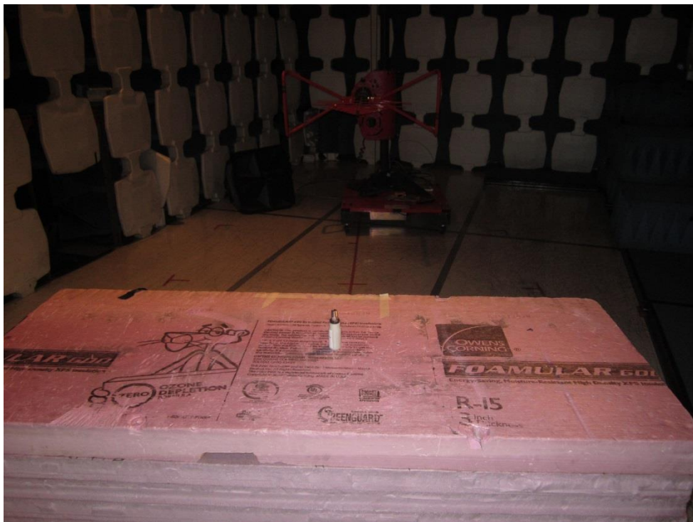
Radiated Emission - Rear 30-1000MHz
