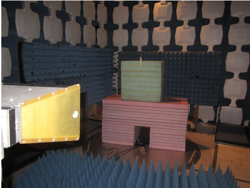
Radiated Emission - Front 1-6GHz
