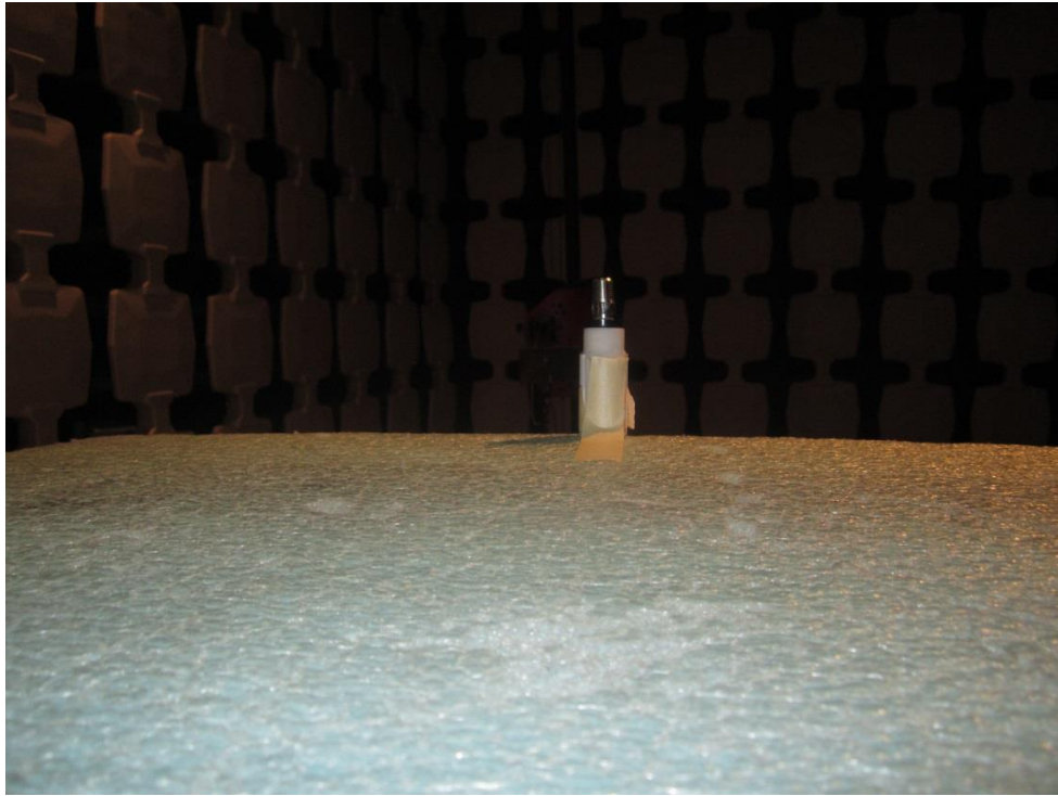
Radiated Emission - 6-18GHz
