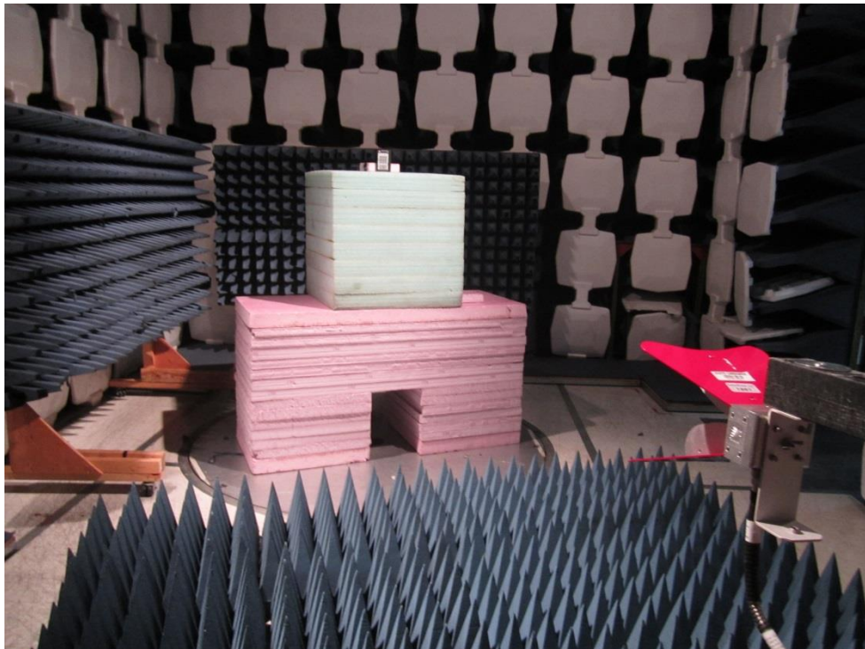
REMI 1-6GHz front
