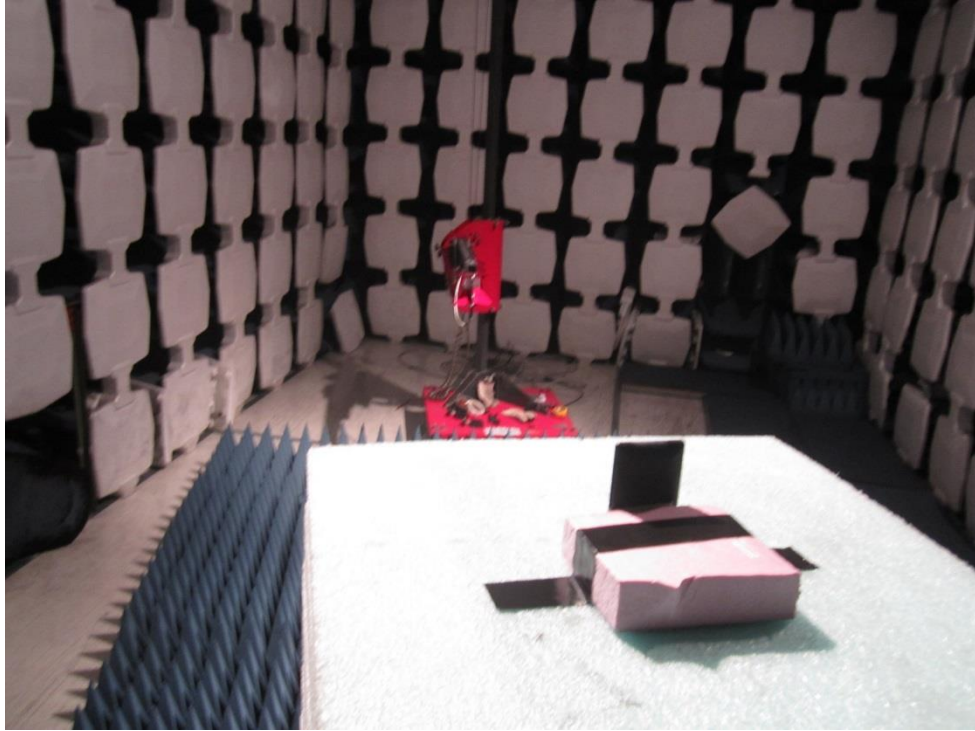
REMI 1-6GHz rear
