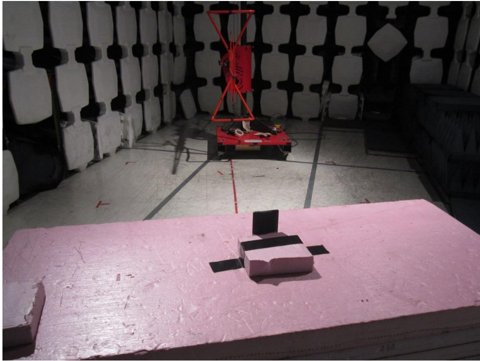
REMI 30-1000MHz rear
