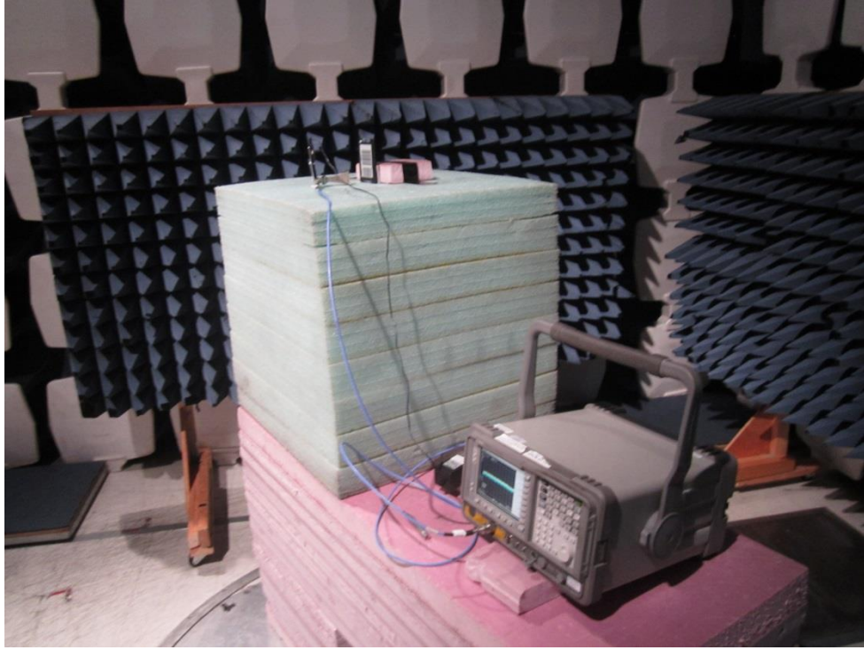
REMI 18-25GHz setup
