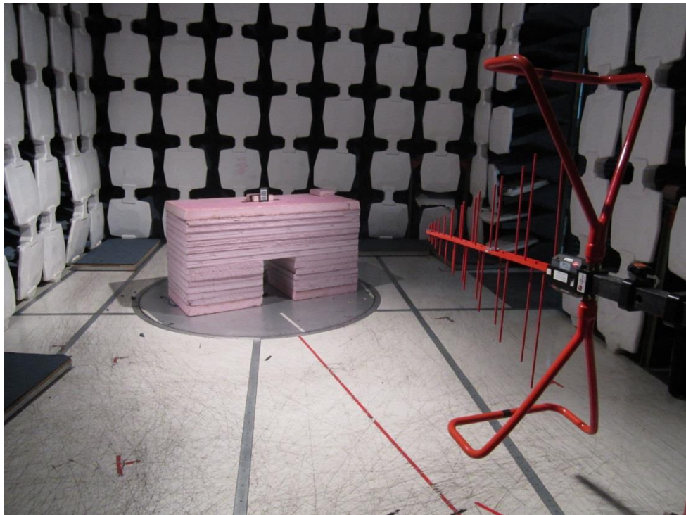
REMI 30-1000MHz front
