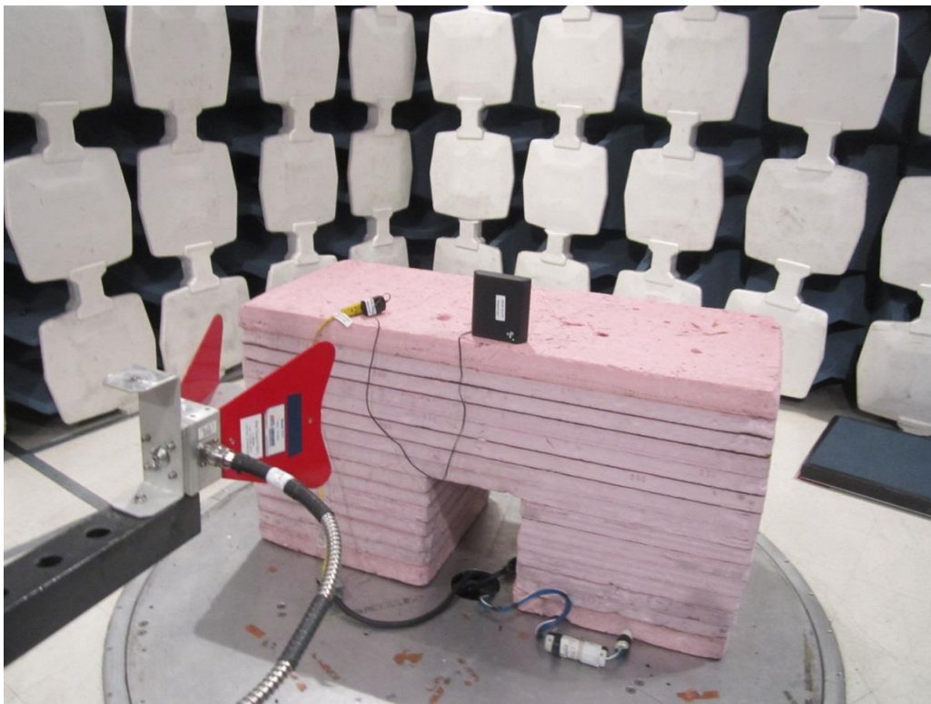
6-10GHz
