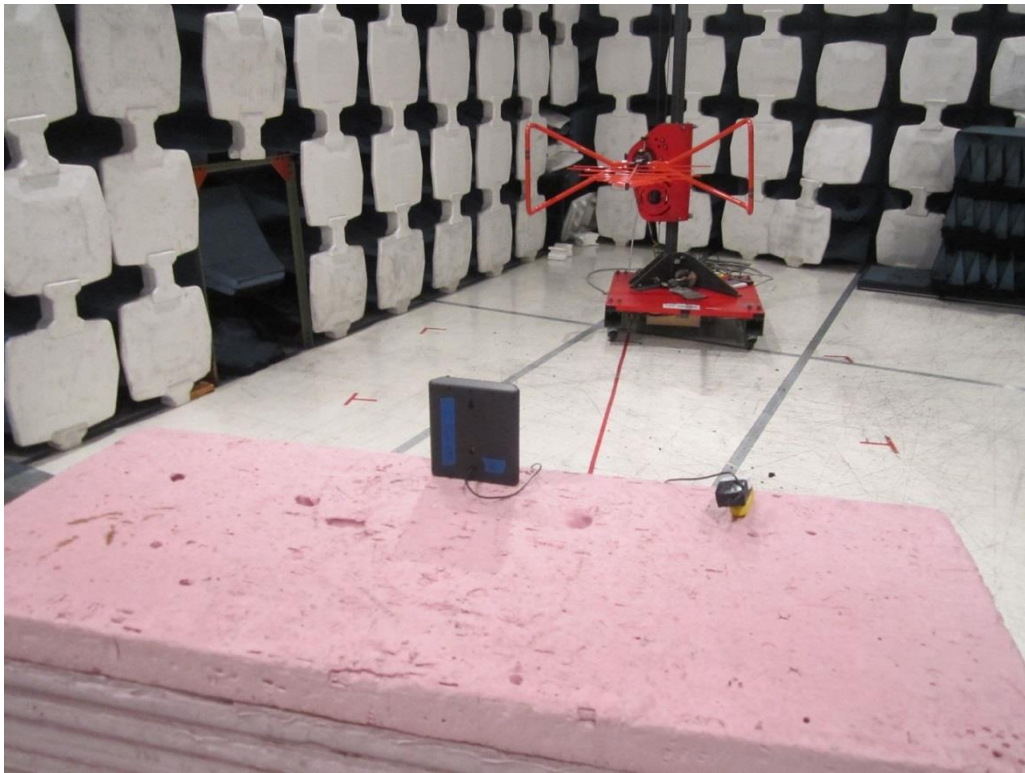
30-1000MHz - Rear
