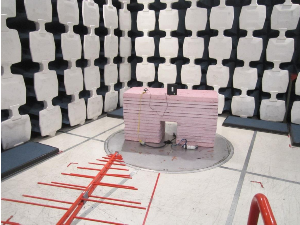
30-1000MHz - Front
