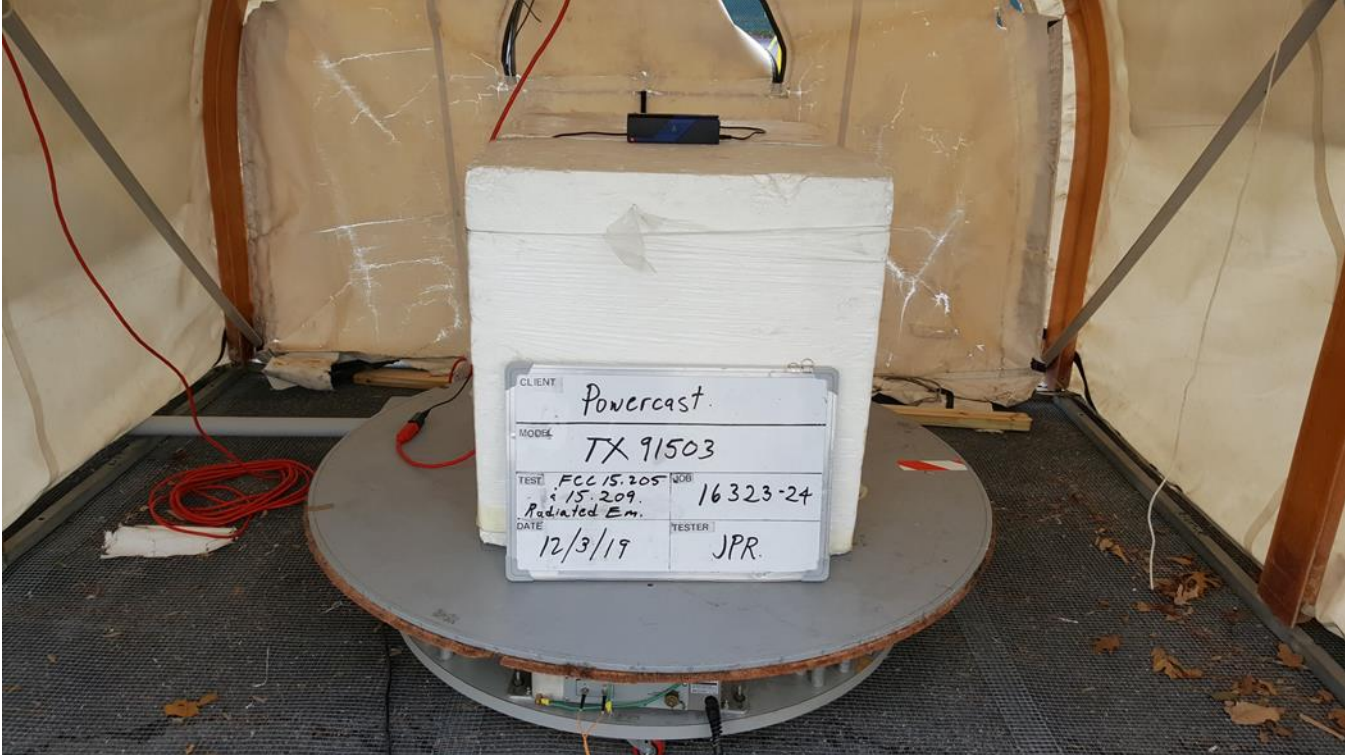
Photograph 3: Radiated Emissions Test Configuration - Side
