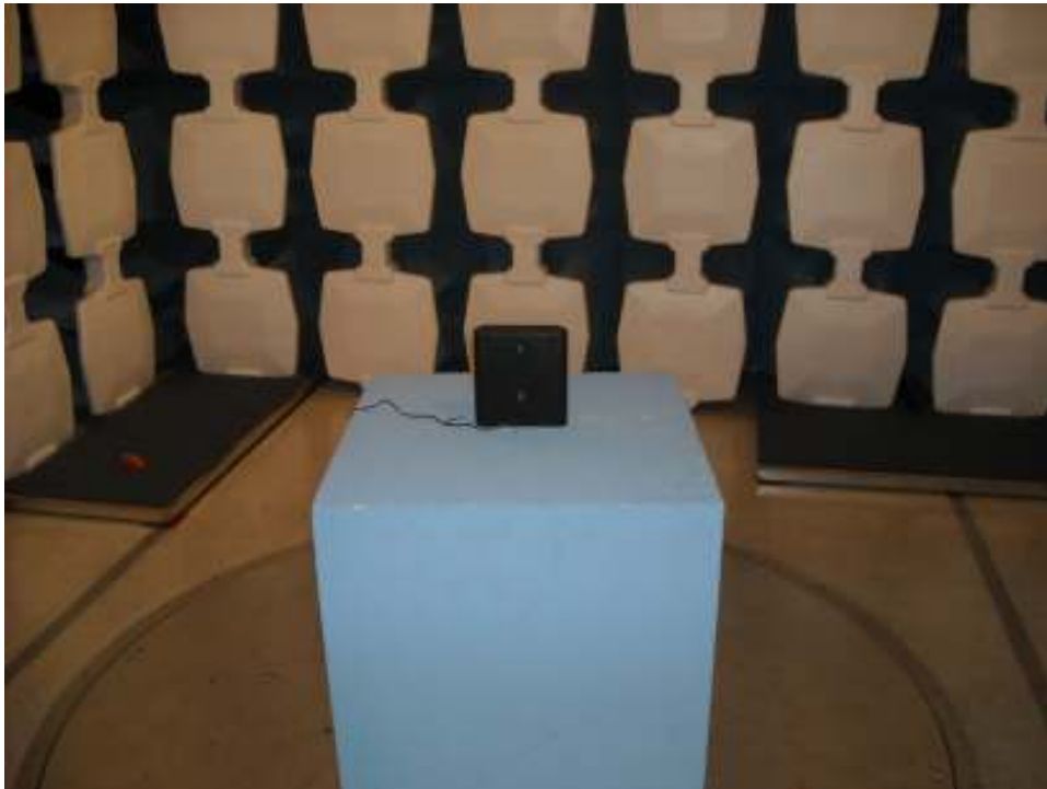
Radiated Emissions – Below 1GHz – Wall Mount
