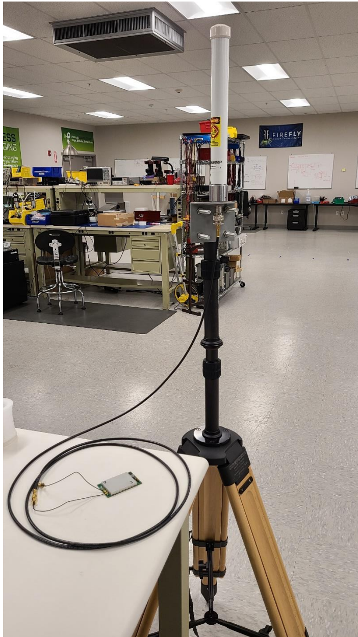
Pasternack PE51OM1013, omnidirectional dipole antenna, gain = 3dBi
