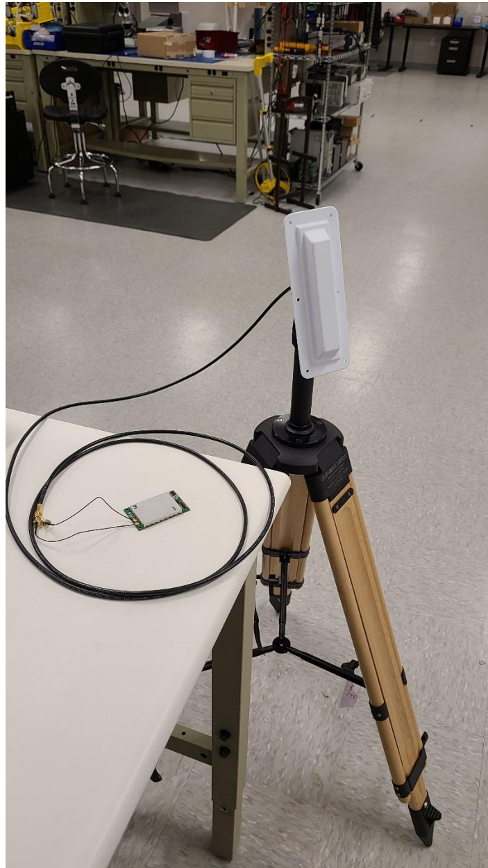
Powercast PAP-ANT-H1-915, linearly polarized patch antenna, gain = 6 dBi
