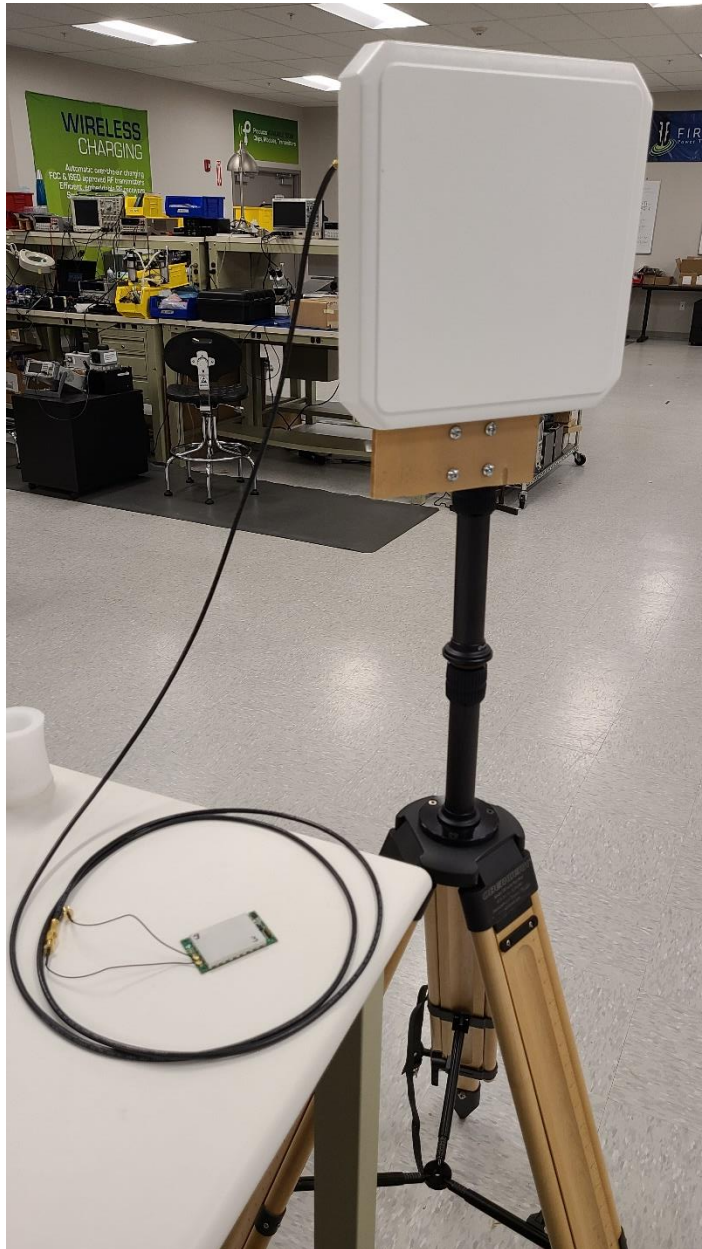
Laird PAR90209H, circularly polarized panel antenna, gain = 9 dBi = 6 dBi
