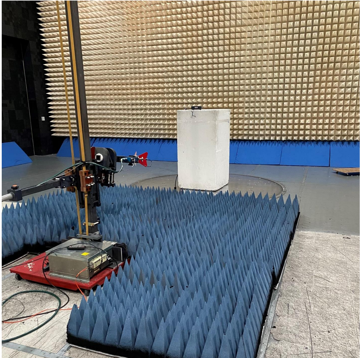
Radiated spurious emissions, 1GHz – 18GHz
