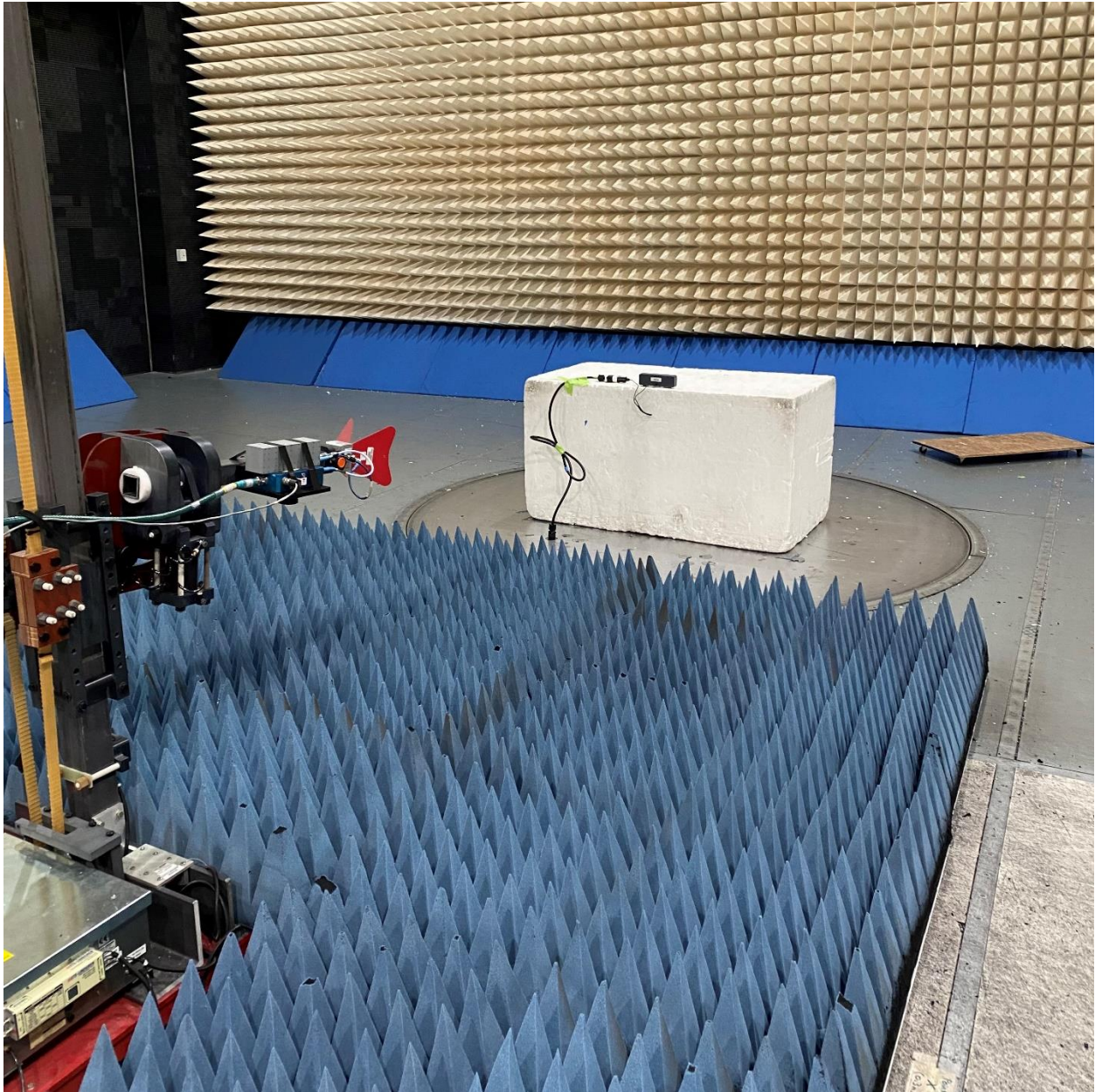
Unintentional emissions, 1GHz – 18GHz
