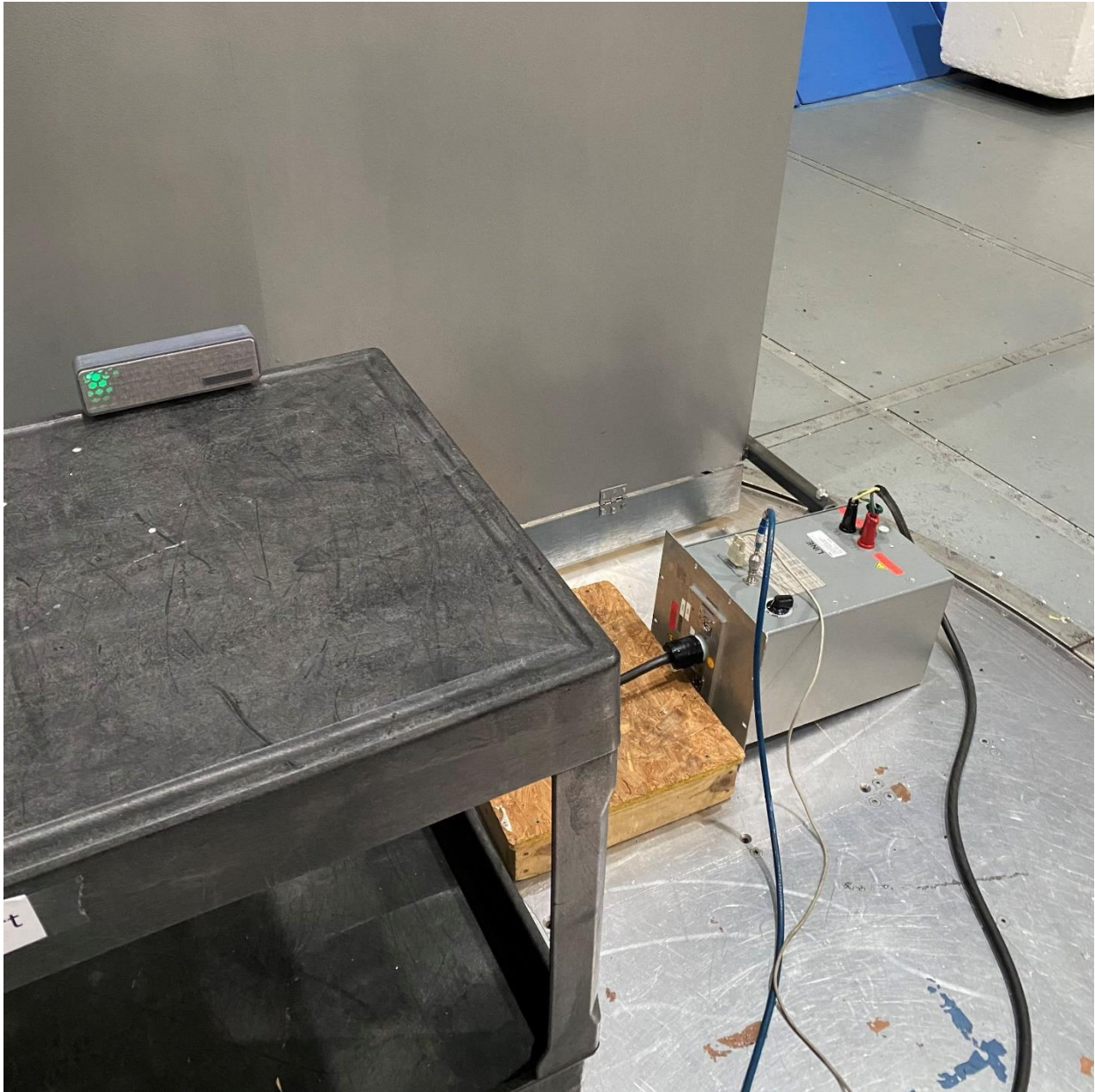
Conducted emissions 150kHz – 30MHz
