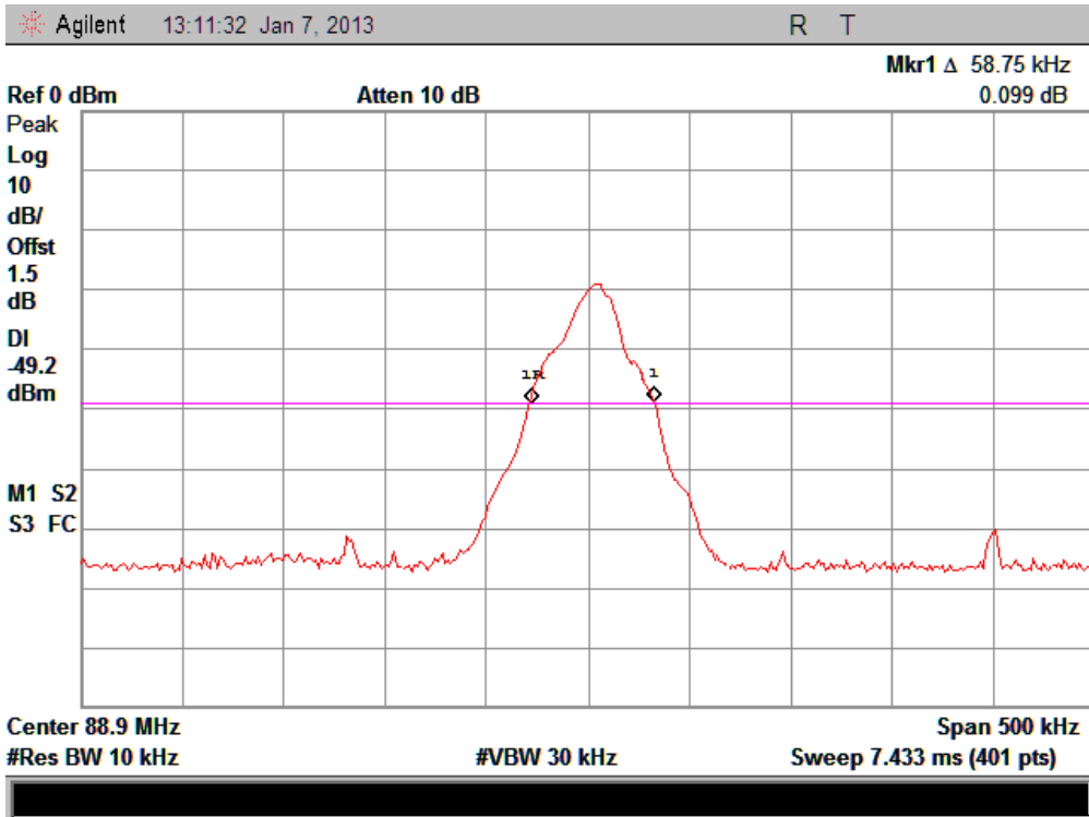
88.9MHz bandwidth test plot
