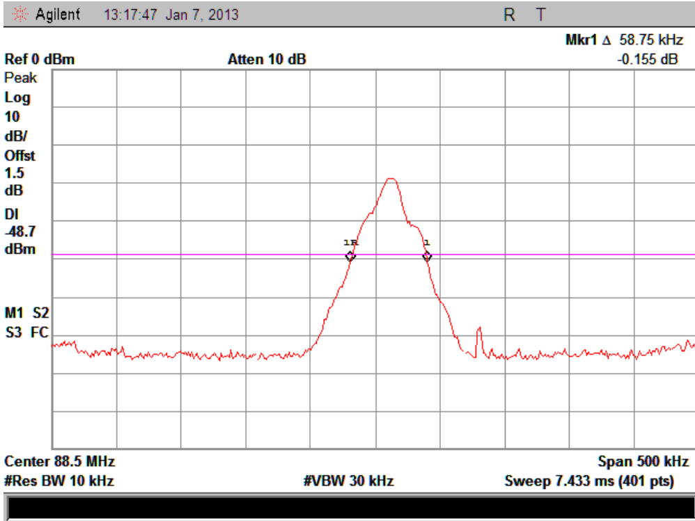
88.5MHz bandwidth test plot
