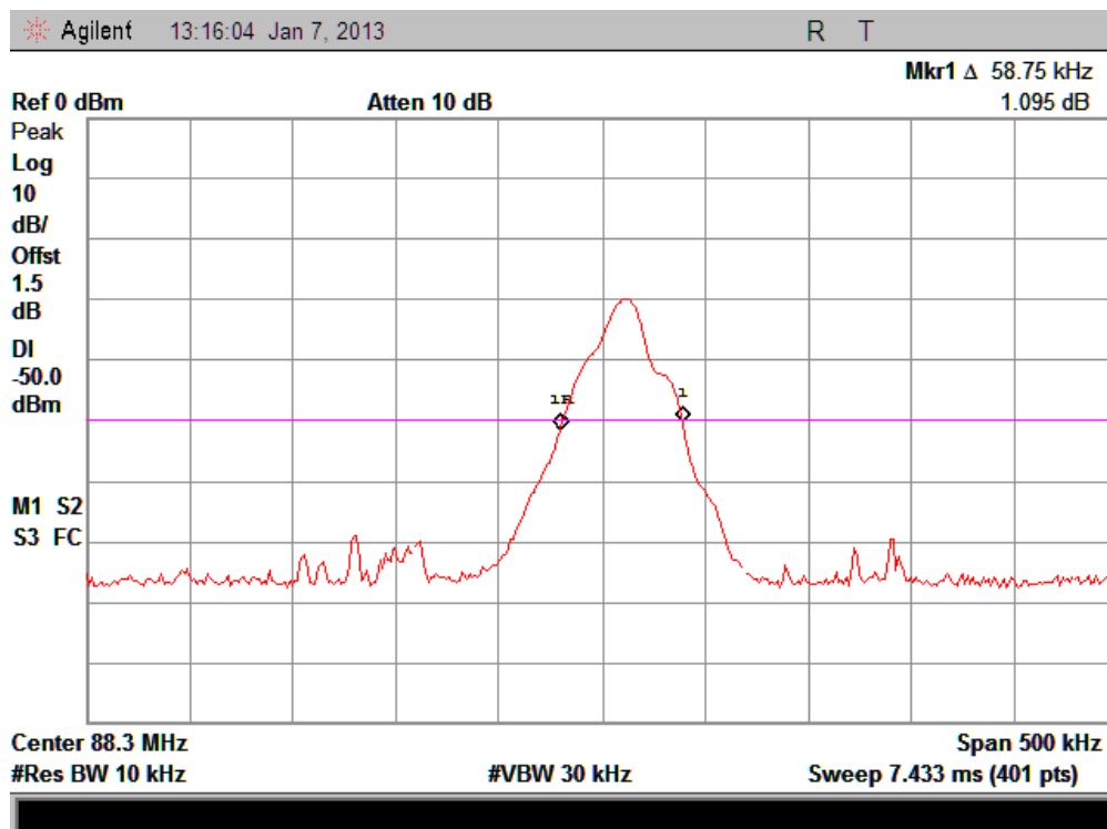
88.3MHz bandwidth test plot
