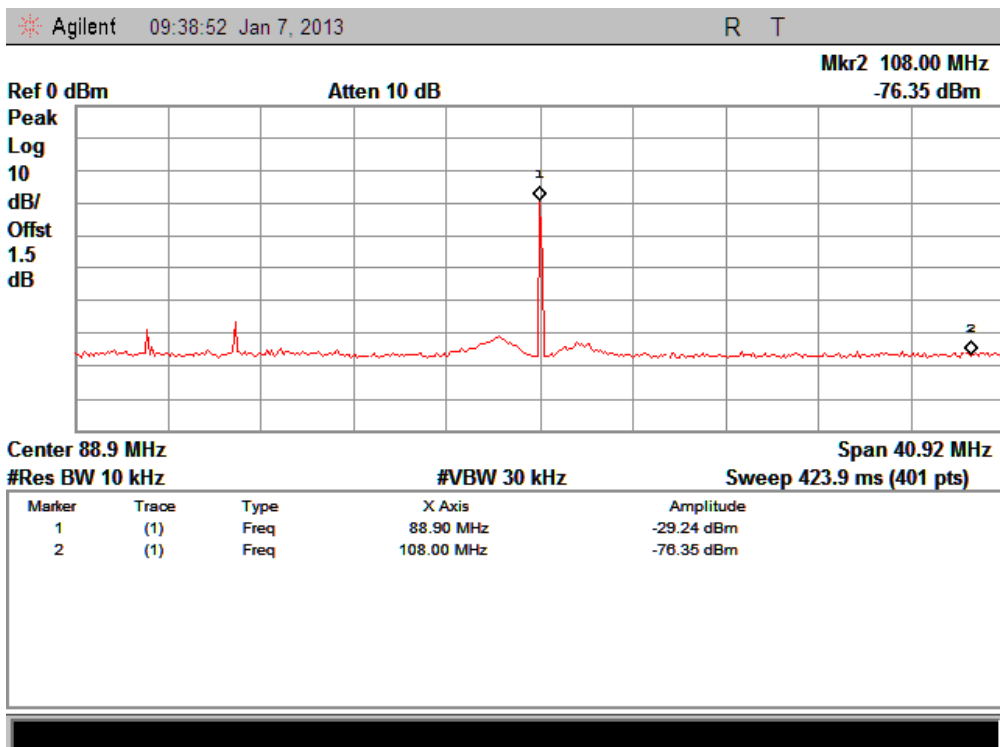
88.9MHz Test Plot
