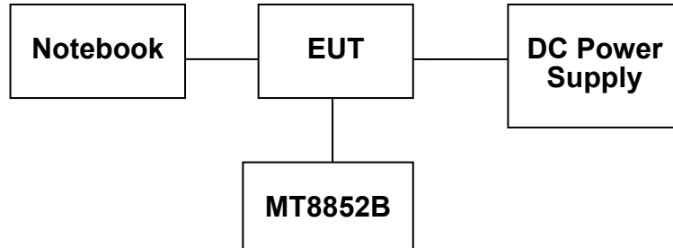
Fig. 2-1 Radiated Emission
