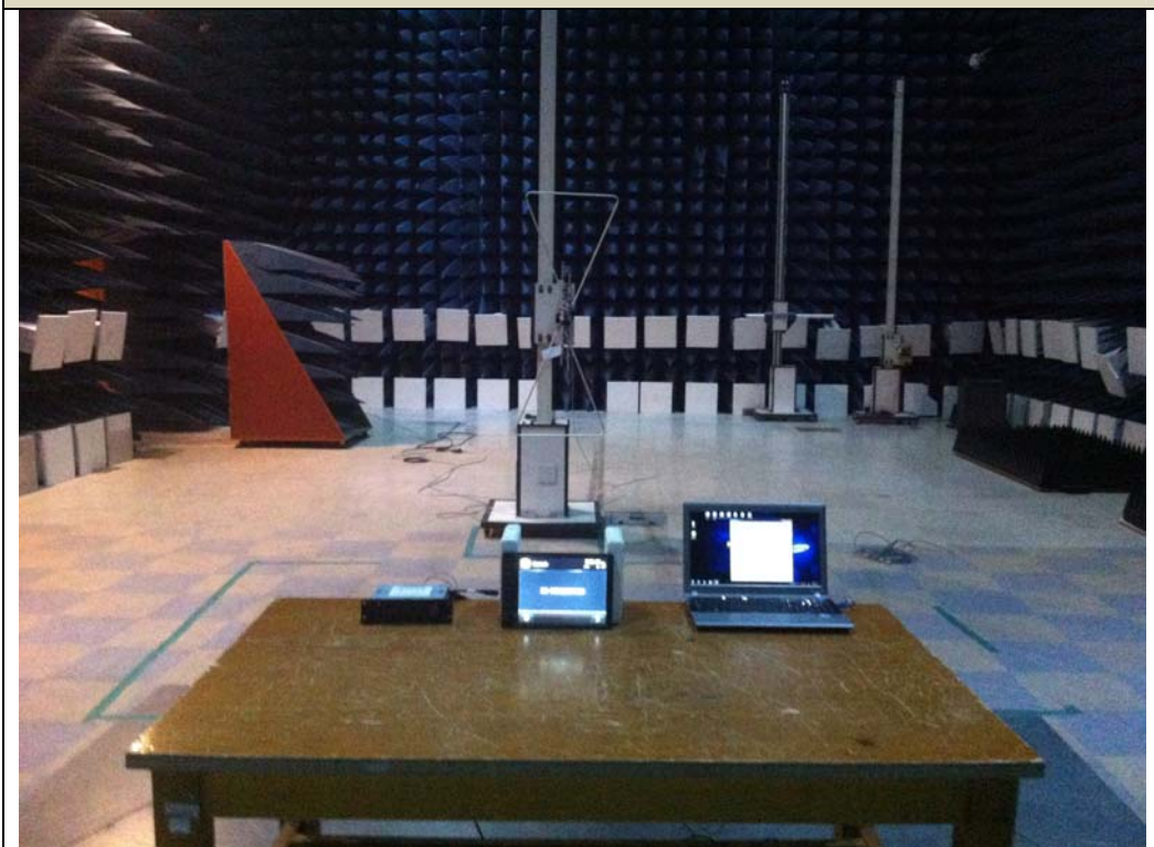
Radiated Spurious Emission<30 MHz to 1 GHz>
