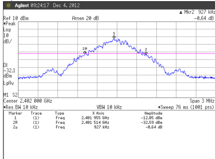
Figure 3. Plot of the 20 dB Channel Bandwidth
