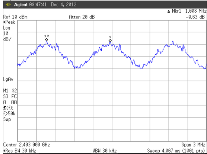
Figure 2. Plot of the Carrier Frequency Separation
