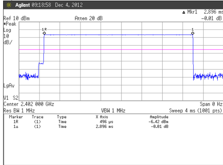
Figure 5. Plot of the Time of Occupancy
