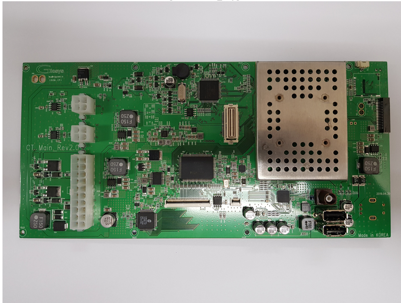
[Main Board_Top]
