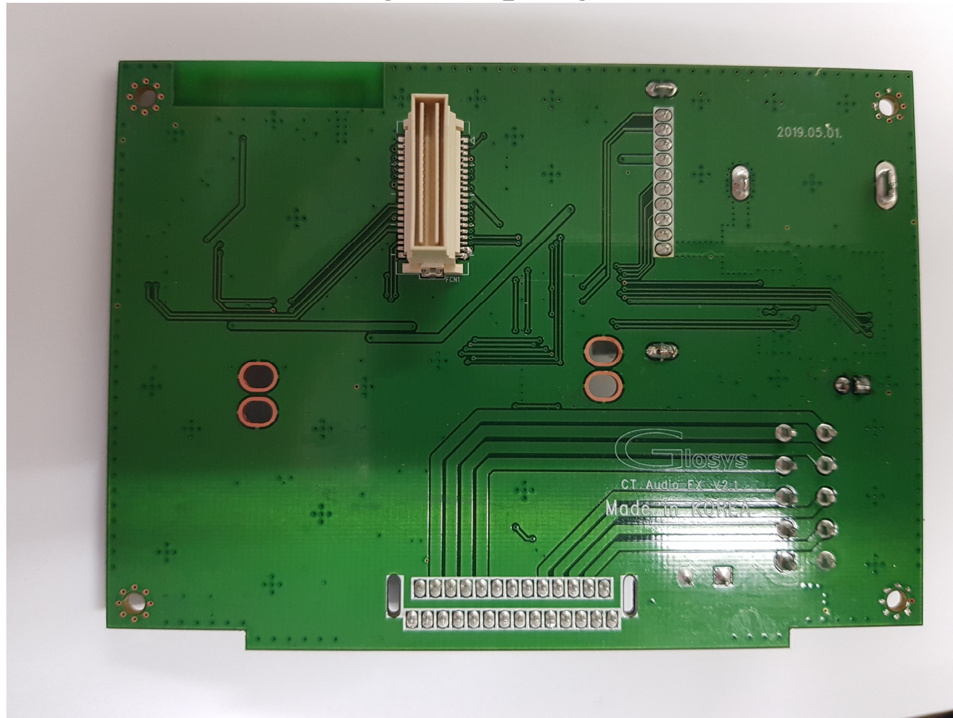
[Audio Board_Bottom]
