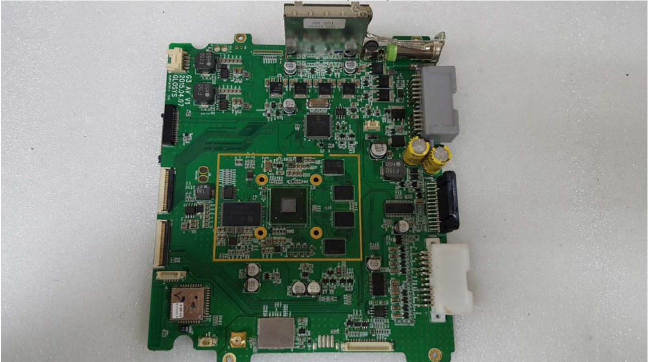
Main Board(back)
