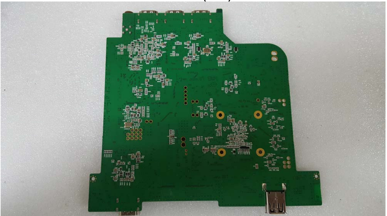
Sub Board(back)
