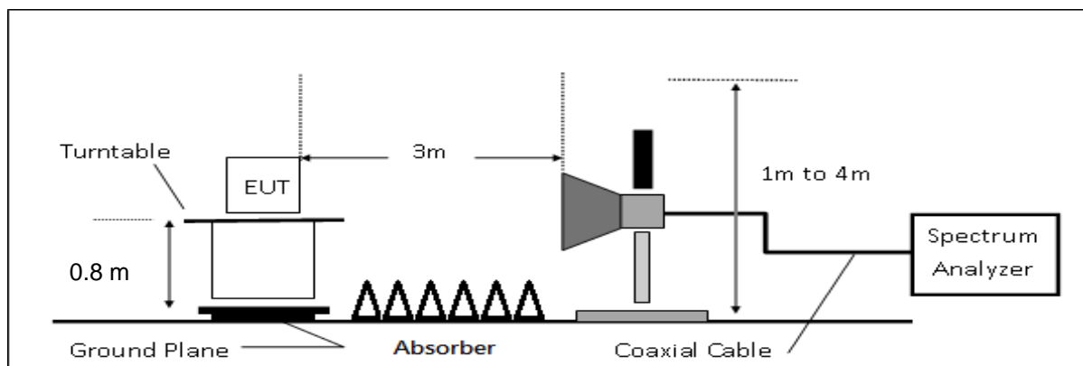
(C) Radiated Emission Test Set-UP Frequency Over 1 GHz
