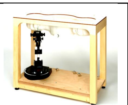
Fig 5.8 Photo of SAM Phantom
