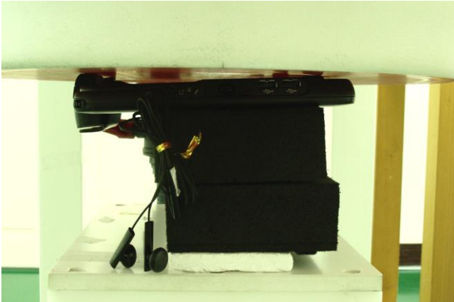
Bottom of DUT Touching with Phantom 0 cm Gap (DUT + Battery 1)
