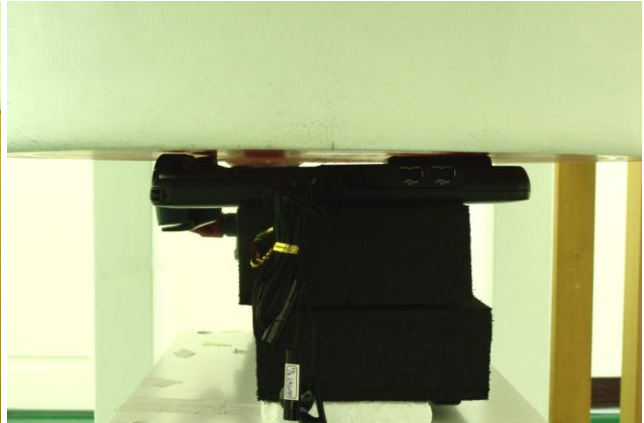
Bottom of DUT Touching with Phantom 0 cm Gap (DUT + Battery 2)
